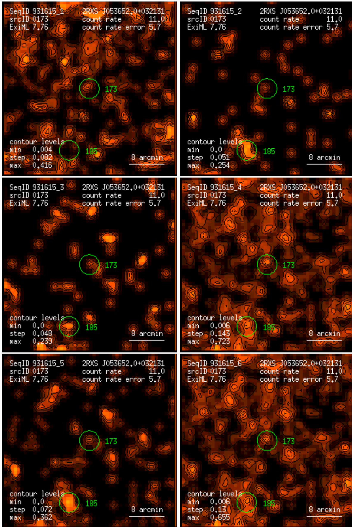
Figure 173: RASS 931615: detection 0173: band rate images, Gaussian filter: (1) PSPC channels 11 – 41, (2) 52 – 90, (3) 91 – 201, (4) 11 – 235, (5) 52 – 201, (6) 11 – 201. Broad band rates in counts/ks. Band rate contour levels in counts/ks/arcmin 2 .
