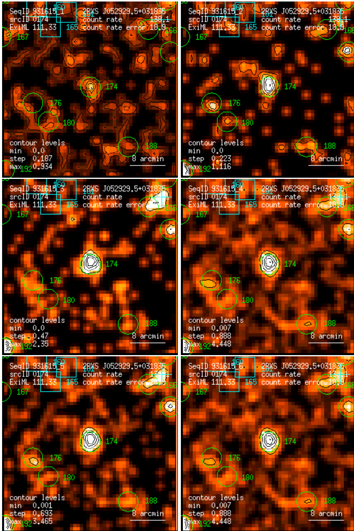
Figure 174: RASS 931615: detection 0174: band rate images, Gaussian filter: (1) PSPC channels 11 – 41, (2) 52 – 90, (3) 91 – 201, (4) 11 – 235, (5) 52 – 201, (6) 11 – 201. Broad band rates in counts/ks. Band rate contour levels in counts/ks/arcmin 2 .
