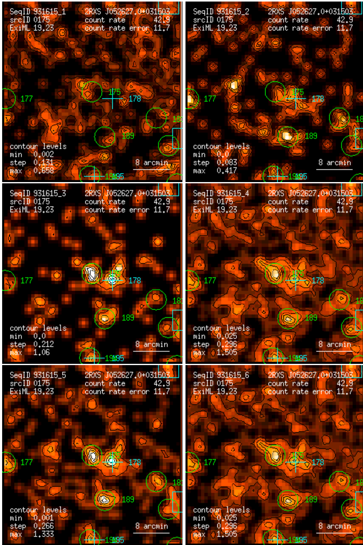
Figure 175: RASS 931615: detection 0175: band rate images, Gaussian filter: (1) PSPC channels 11 – 41, (2) 52 – 90, (3) 91 – 201, (4) 11 – 235, (5) 52 – 201, (6) 11 – 201. Broad band rates in counts/ks. Band rate contour levels in counts/ks/arcmin 2 .
