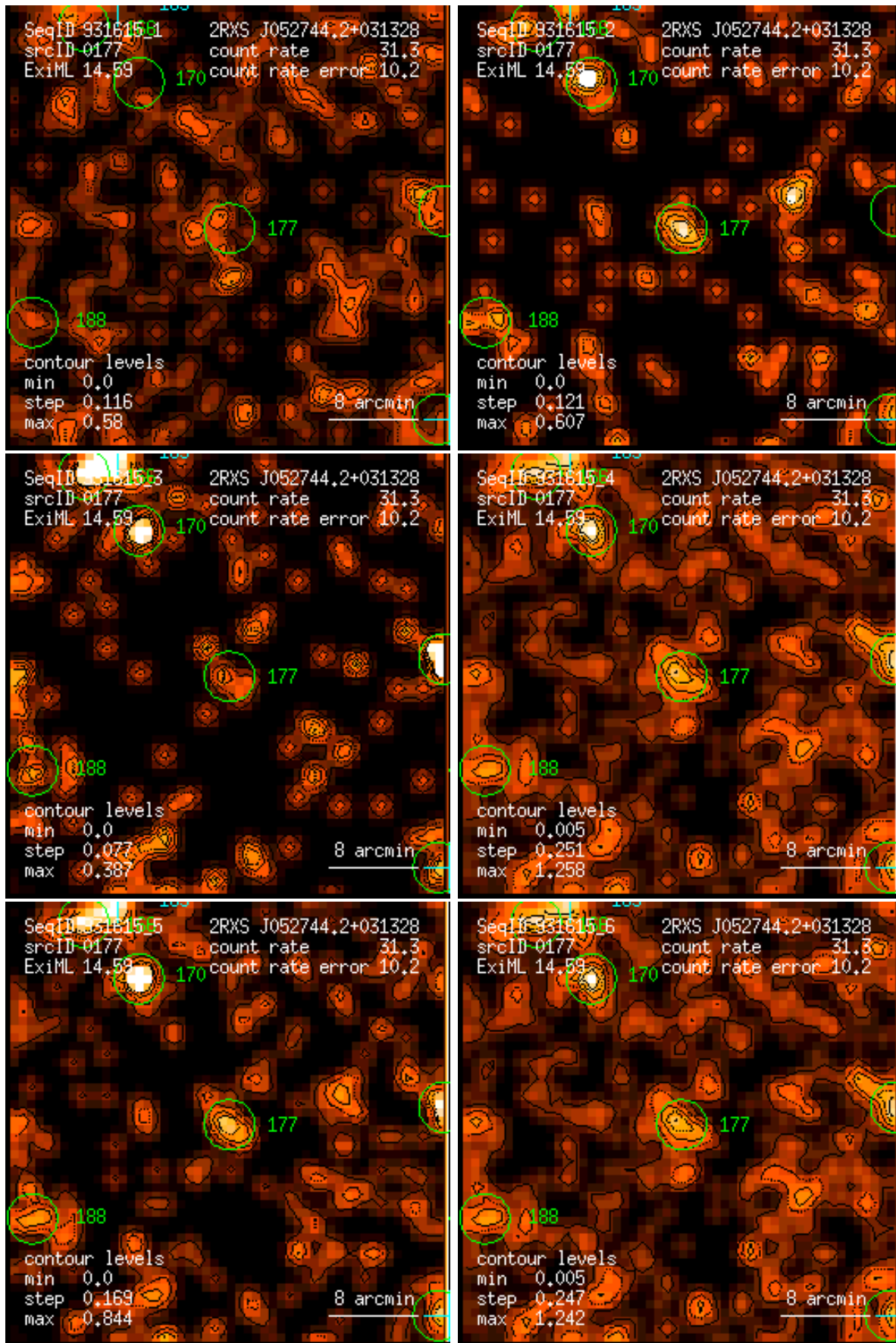
Figure 177: RASS 931615: detection 0177: band rate images, Gaussian filter: (1) PSPC channels 11 – 41, (2) 52 – 90, (3) 91 – 201, (4) 11 – 235, (5) 52 – 201, (6) 11 – 201. Broad band rates in counts/ks. Band rate contour levels in counts/ks/arcmin 2 .
