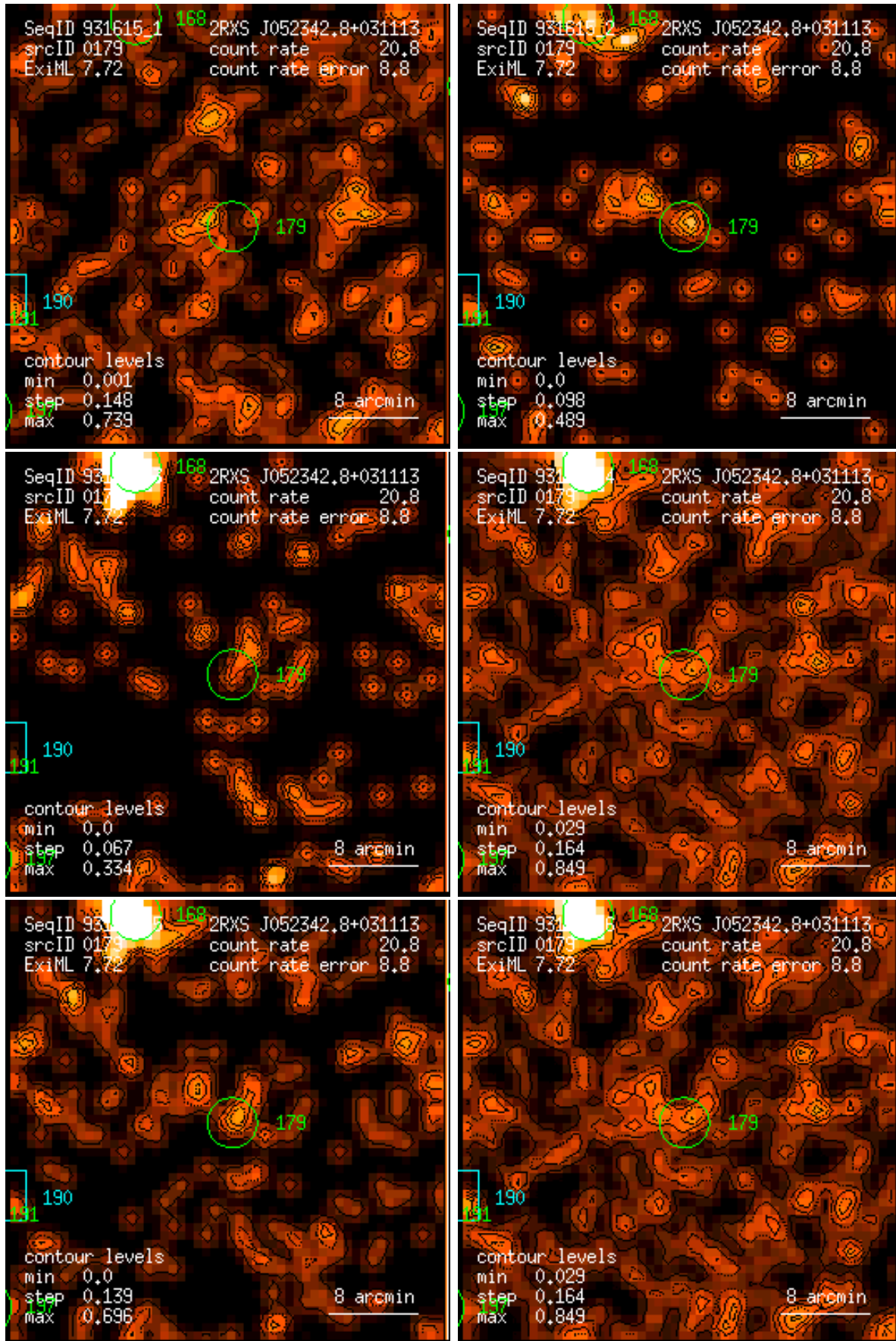
Figure 179: RASS 931615: detection 0179: band rate images, Gaussian filter: (1) PSPC channels 11 – 41, (2) 52 – 90, (3) 91 – 201, (4) 11 – 235, (5) 52 – 201, (6) 11 – 201. Broad band rates in counts/ks. Band rate contour levels in counts/ks/arcmin 2 .
