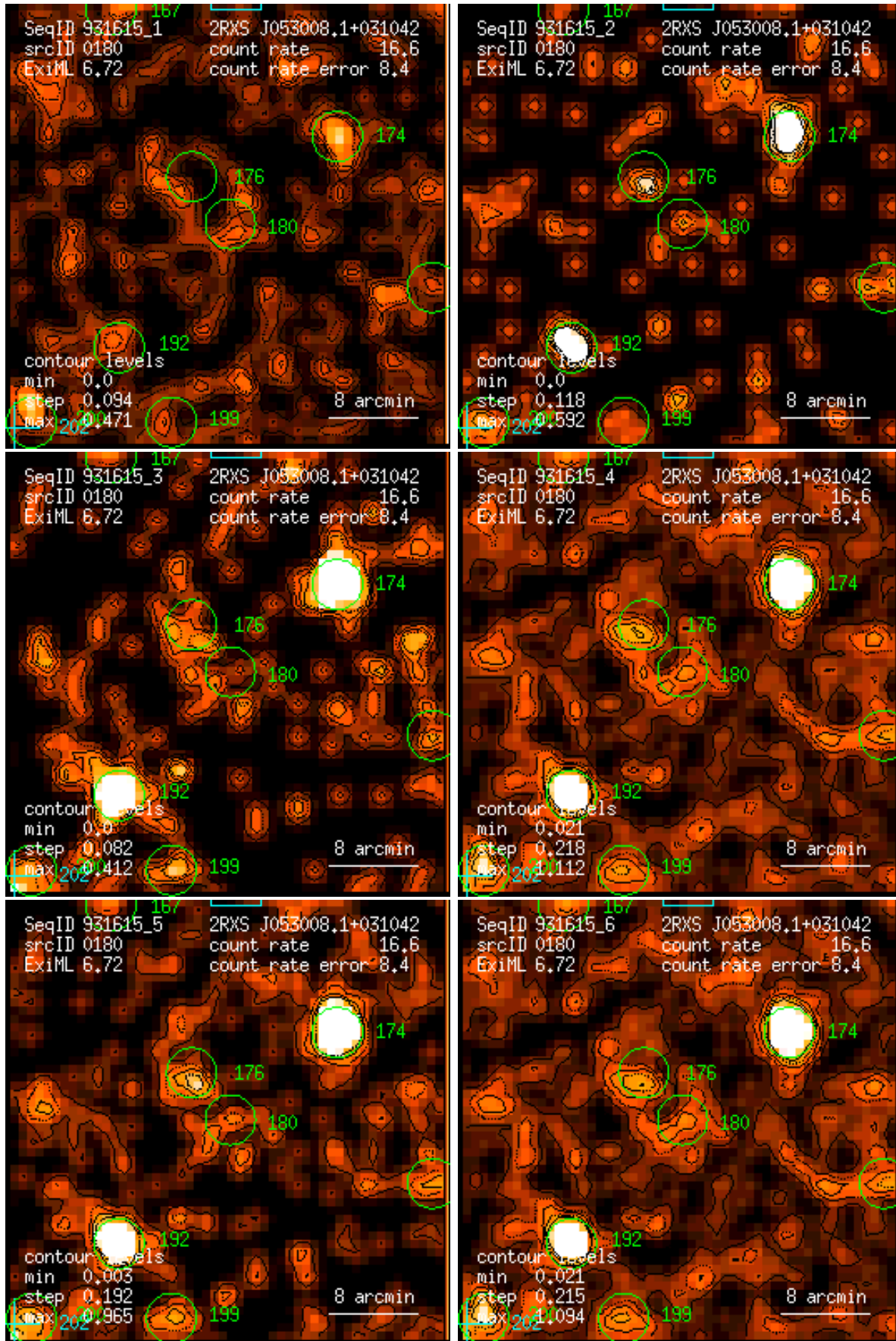
Figure 180: RASS 931615: detection 0180: band rate images, Gaussian filter: (1) PSPC channels 11 – 41, (2) 52 – 90, (3) 91 – 201, (4) 11 – 235, (5) 52 – 201, (6) 11 – 201. Broad band rates in counts/ks. Band rate contour levels in counts/ks/arcmin 2 .
