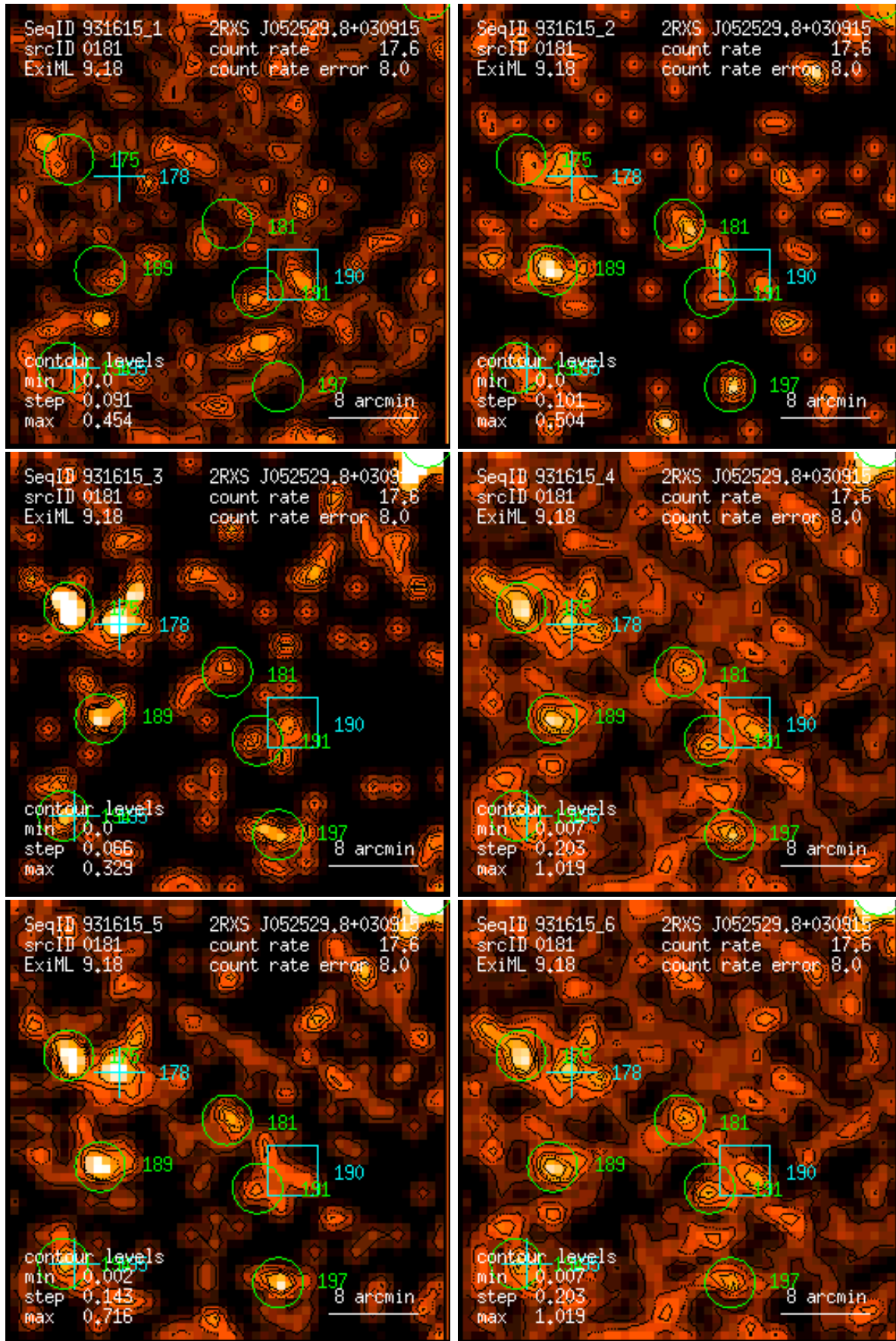
Figure 181: RASS 931615: detection 0181: band rate images, Gaussian filter: (1) PSPC channels 11 – 41, (2) 52 – 90, (3) 91 – 201, (4) 11 – 235, (5) 52 – 201, (6) 11 – 201. Broad band rates in counts/ks. Band rate contour levels in counts/ks/arcmin 2 .
