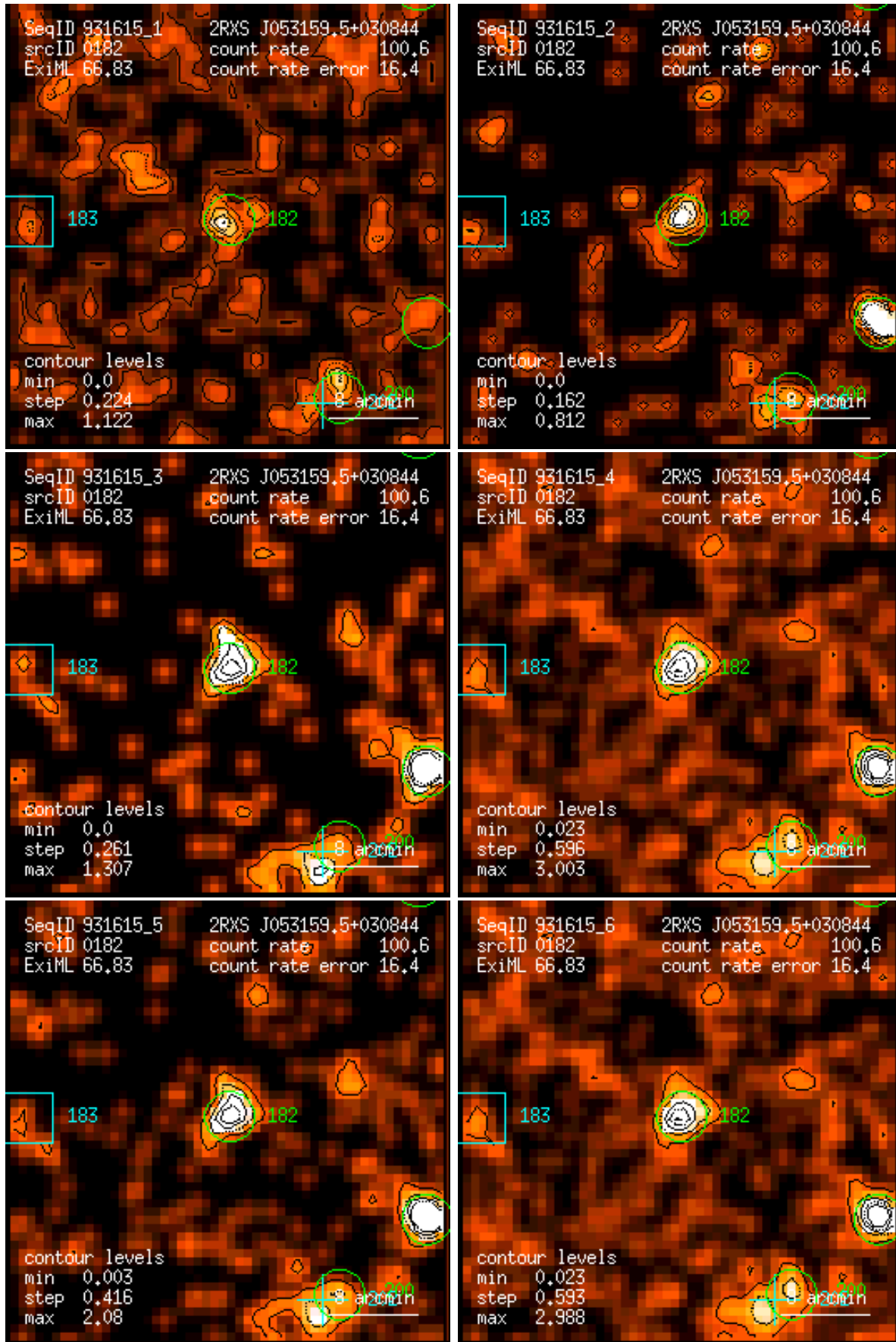
Figure 182: RASS 931615: detection 0182: band rate images, Gaussian filter: (1) PSPC channels 11 – 41, (2) 52 – 90, (3) 91 – 201, (4) 11 – 235, (5) 52 – 201, (6) 11 – 201. Broad band rates in counts/ks. Band rate contour levels in counts/ks/arcmin 2 .
