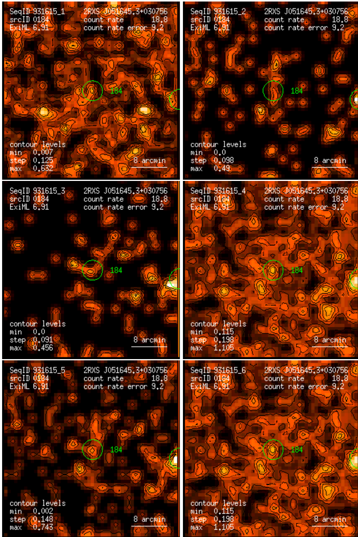
Figure 184: RASS 931615: detection 0184: band rate images, Gaussian filter: (1) PSPC channels 11 – 41, (2) 52 – 90, (3) 91 – 201, (4) 11 – 235, (5) 52 – 201, (6) 11 – 201. Broad band rates in counts/ks. Band rate contour levels in counts/ks/arcmin 2 .
