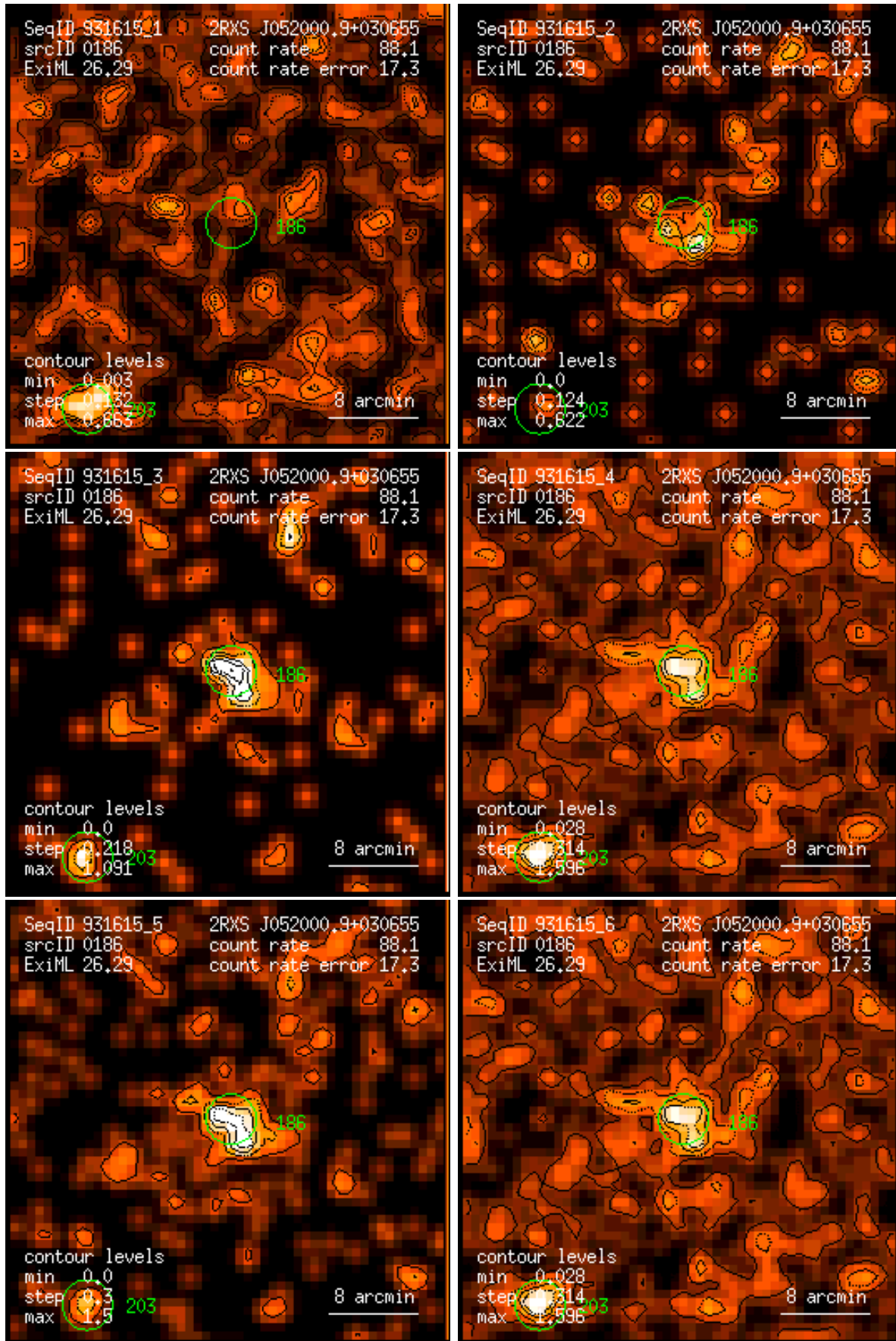
Figure 186: RASS 931615: detection 0186: band rate images, Gaussian filter: (1) PSPC channels 11 – 41, (2) 52 – 90, (3) 91 – 201, (4) 11 – 235, (5) 52 – 201, (6) 11 – 201. Broad band rates in counts/ks. Band rate contour levels in counts/ks/arcmin 2 .
