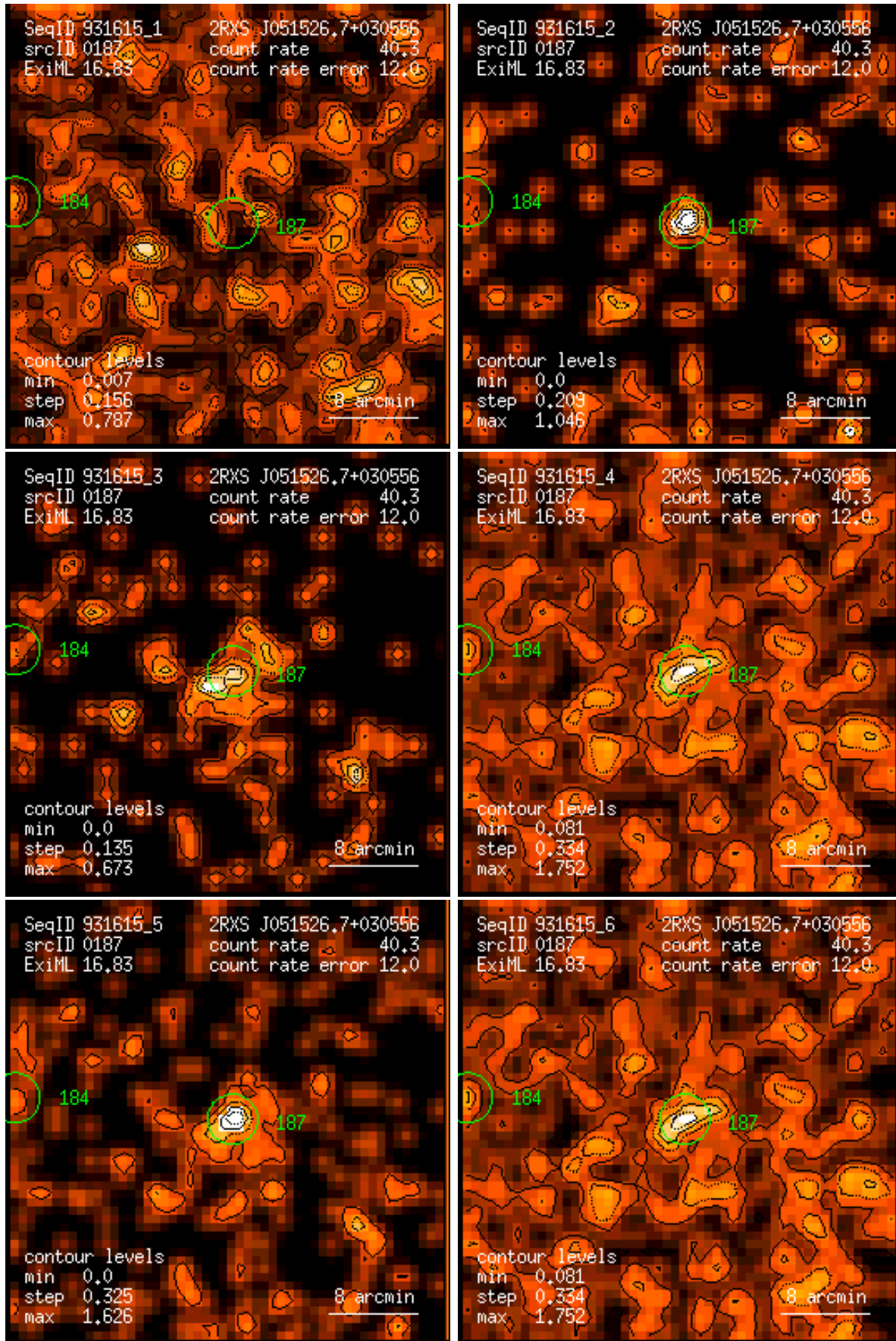
Figure 187: RASS 931615: detection 0187: band rate images, Gaussian filter: (1) PSPC channels 11 – 41, (2) 52 – 90, (3) 91 – 201, (4) 11 – 235, (5) 52 – 201, (6) 11 – 201. Broad band rates in counts/ks. Band rate contour levels in counts/ks/arcmin 2 .
