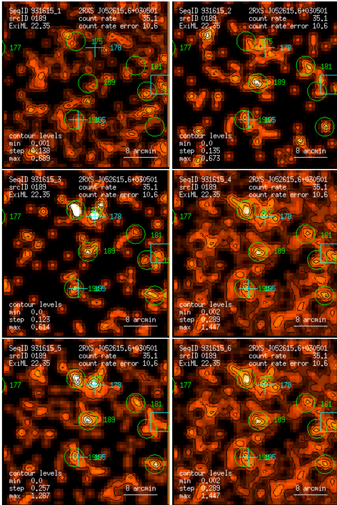
Figure 189: RASS 931615: detection 0189: band rate images, Gaussian filter: (1) PSPC channels 11 – 41, (2) 52 – 90, (3) 91 – 201, (4) 11 – 235, (5) 52 – 201, (6) 11 – 201. Broad band rates in counts/ks. Band rate contour levels in counts/ks/arcmin 2 .
