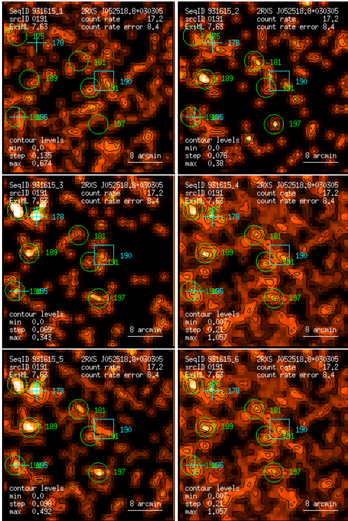
Figure 191: RASS 931615: detection 0191: band rate images, Gaussian filter: (1) PSPC channels 11 – 41, (2) 52 – 90, (3) 91 – 201, (4) 11 – 235, (5) 52 – 201, (6) 11 – 201. Broad band rates in counts/ks. Band rate contour levels in counts/ks/arcmin 2 .
