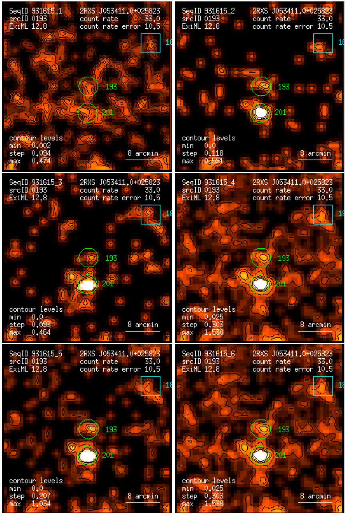
Figure 193: RASS 931615: detection 0193: band rate images, Gaussian filter: (1) PSPC channels 11 – 41, (2) 52 – 90, (3) 91 – 201, (4) 11 – 235, (5) 52 – 201, (6) 11 – 201. Broad band rates in counts/ks. Band rate contour levels in counts/ks/arcmin 2 .
