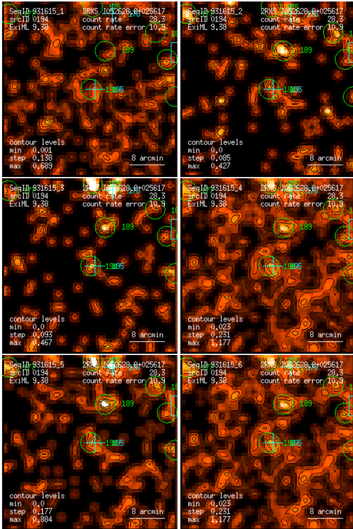
Figure 194: RASS 931615: detection 0194: band rate images, Gaussian filter: (1) PSPC channels 11 – 41, (2) 52 – 90, (3) 91 – 201, (4) 11 – 235, (5) 52 – 201, (6) 11 – 201. Broad band rates in counts/ks. Band rate contour levels in counts/ks/arcmin 2 .
