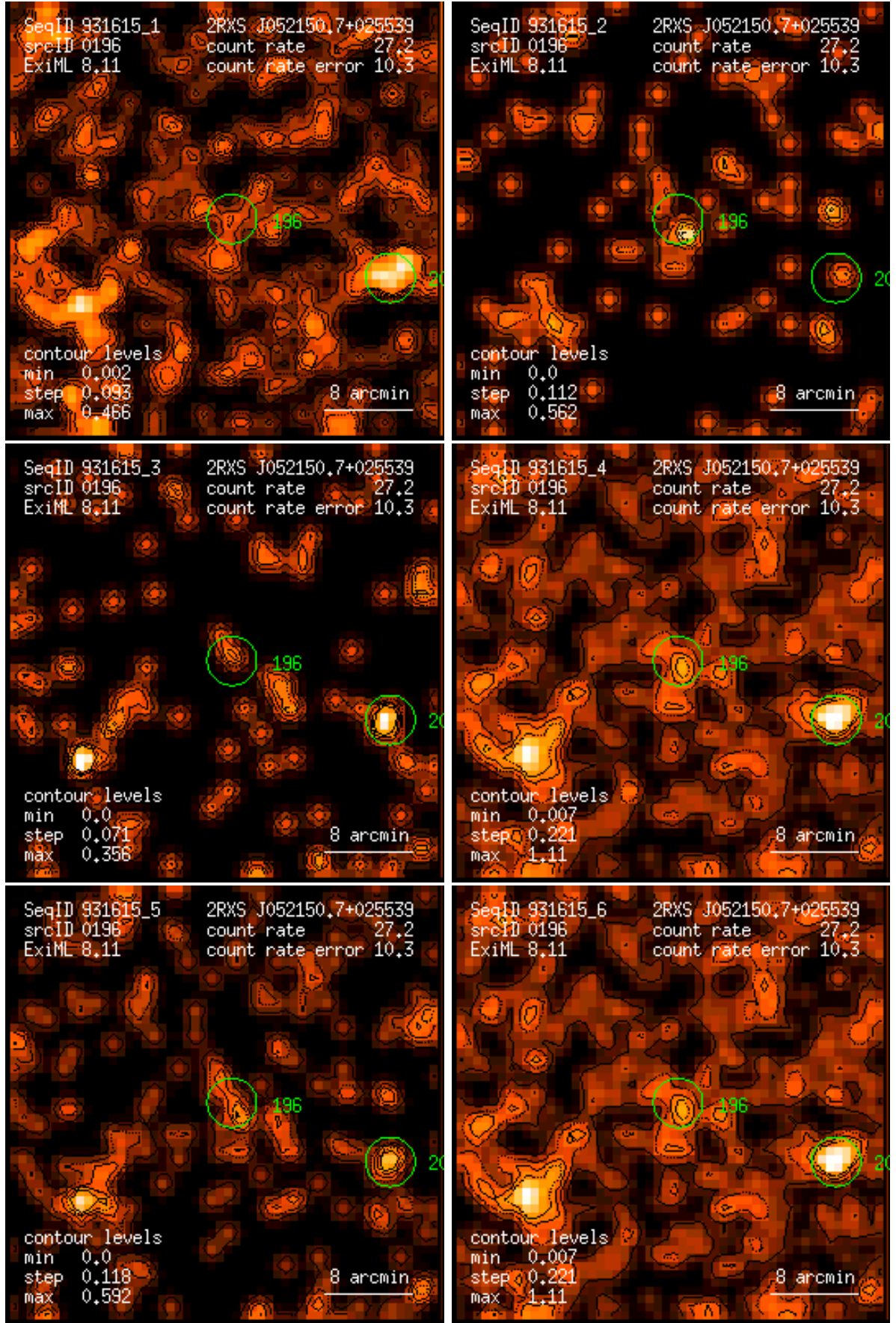
Figure 196: RASS 931615: detection 0196: band rate images, Gaussian filter: (1) PSPC channels 11 – 41, (2) 52 – 90, (3) 91 – 201, (4) 11 – 235, (5) 52 – 201, (6) 11 – 201. Broad band rates in counts/ks. Band rate contour levels in counts/ks/arcmin 2 .
