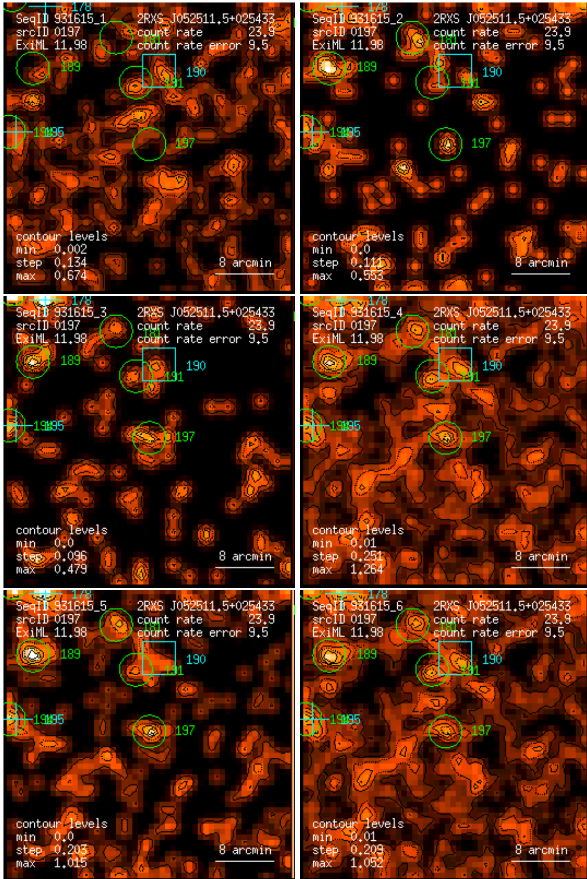
Figure 197: RASS 931615: detection 0197: band rate images, Gaussian filter: (1) PSPC channels 11 – 41, (2) 52 – 90, (3) 91 – 201, (4) 11 – 235, (5) 52 – 201, (6) 11 – 201. Broad band rates in counts/ks. Band rate contour levels in counts/ks/arcmin 2 .
