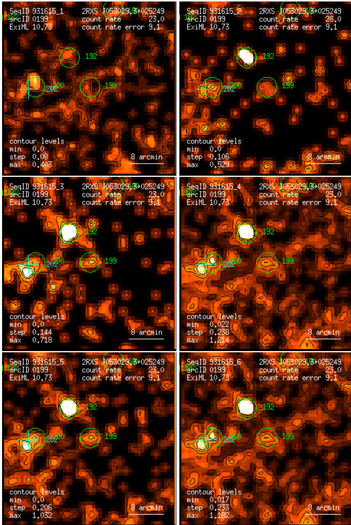
Figure 199: RASS 931615: detection 0199: band rate images, Gaussian filter: (1) PSPC channels 11 – 41, (2) 52 – 90, (3) 91 – 201, (4) 11 – 235, (5) 52 – 201, (6) 11 – 201. Broad band rates in counts/ks. Band rate contour levels in counts/ks/arcmin 2 .
