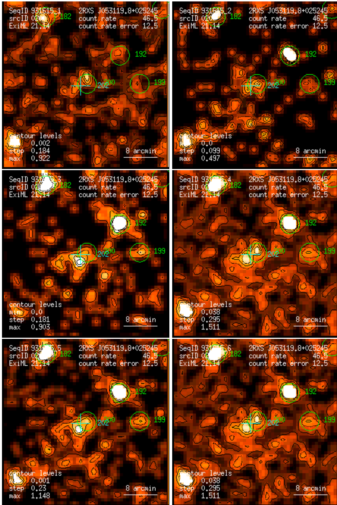
Figure 200: RASS 931615: detection 0200: band rate images, Gaussian filter: (1) PSPC channels 11 – 41, (2) 52 – 90, (3) 91 – 201, (4) 11 – 235, (5) 52 – 201, (6) 11 – 201. Broad band rates in counts/ks. Band rate contour levels in counts/ks/arcmin 2 .
