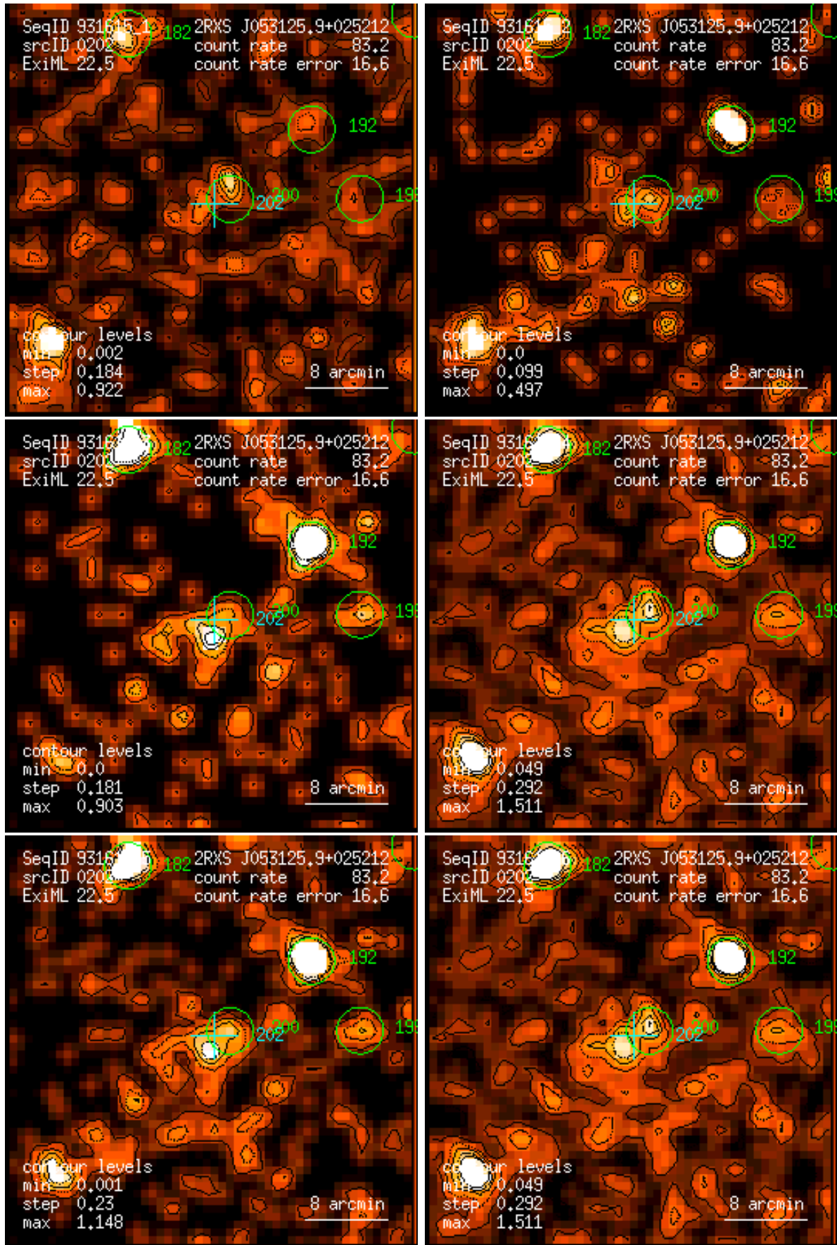
Figure 202: RASS 931615: detection 0202: band rate images, Gaussian filter: (1) PSPC channels 11 – 41, (2) 52 – 90, (3) 91 – 201, (4) 11 – 235, (5) 52 – 201, (6) 11 – 201. Broad band rates in counts/ks. Band rate contour levels in counts/ks/arcmin 2 .
