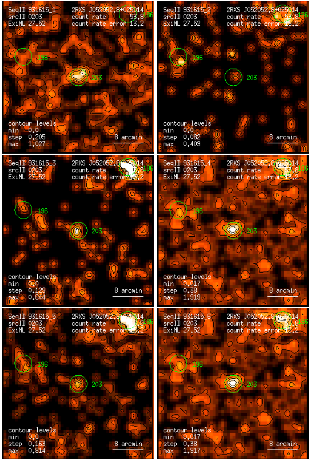
Figure 203: RASS 931615: detection 0203: band rate images, Gaussian filter: (1) PSPC channels 11 – 41, (2) 52 – 90, (3) 91 – 201, (4) 11 – 235, (5) 52 – 201, (6) 11 – 201. Broad band rates in counts/ks. Band rate contour levels in counts/ks/arcmin 2 .
