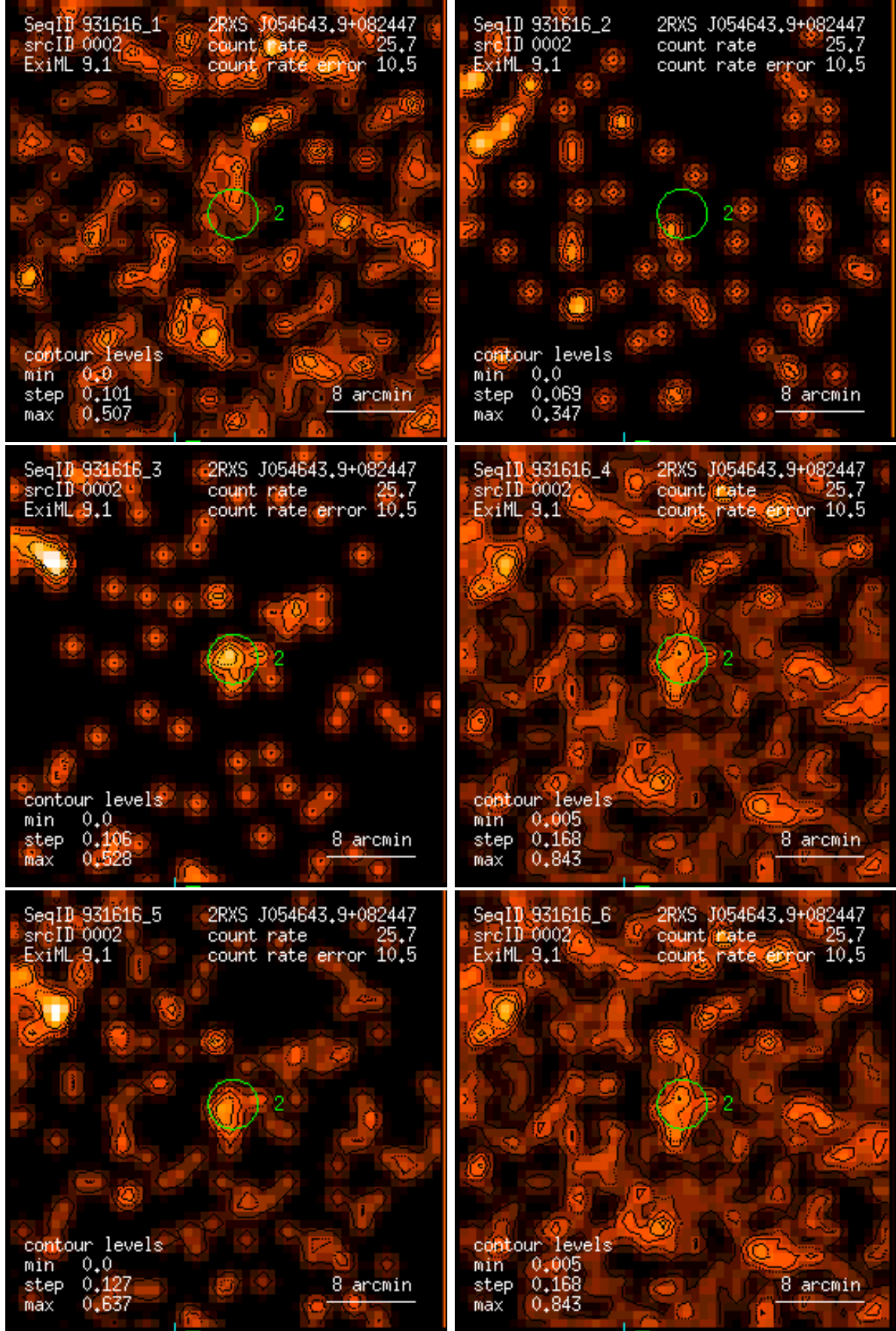
Figure 2: RASS 931616: detection 0002: band rate images, Gaussian filter: (1) PSPC channels 11 – 41, (2) 52 – 90, (3) 91 – 201, (4) 11 – 235, (5) 52 – 201, (6) 11 – 201. Broad band rates in counts/ks. Band rate contour levels in counts/ks/arcmin 2 .
