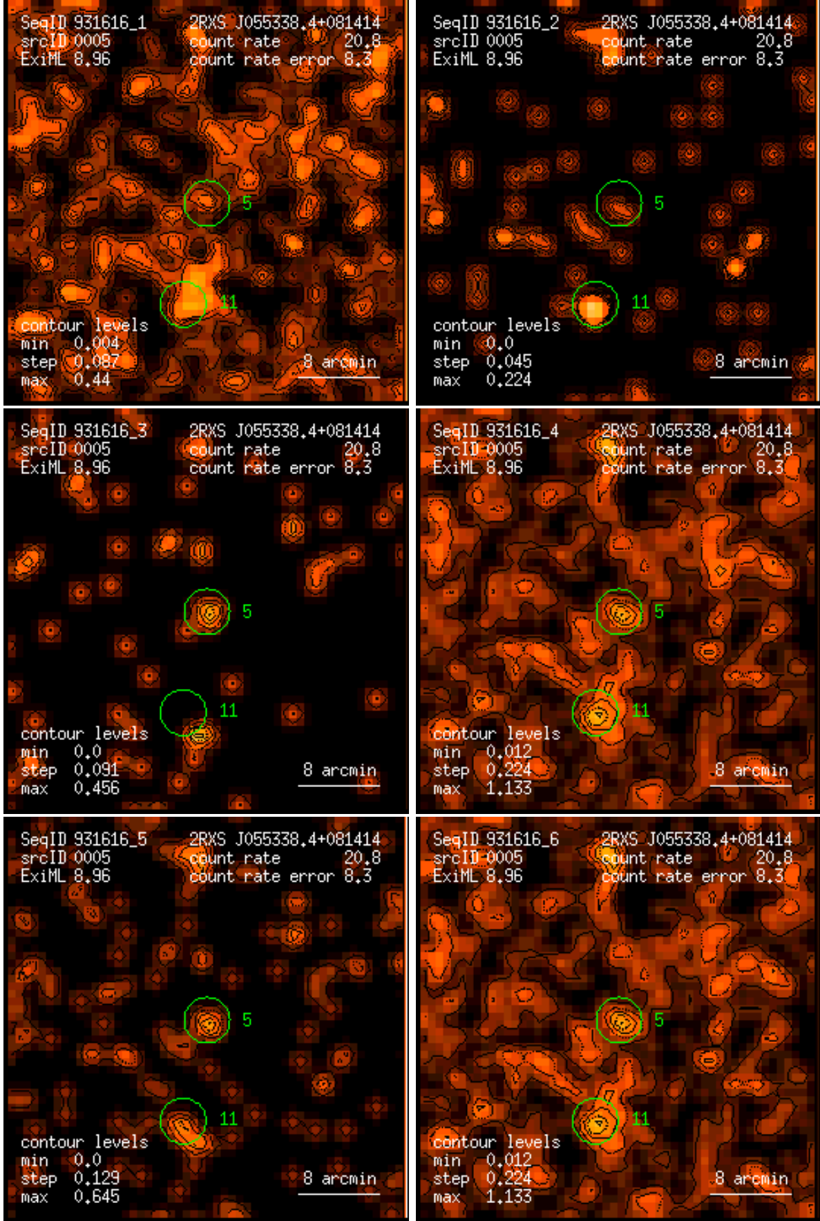
Figure 5: RASS 931616: detection 0005: band rate images, Gaussian filter: (1) PSPC channels 11 – 41, (2) 52 – 90, (3) 91 – 201, (4) 11 – 235, (5) 52 – 201, (6) 11 – 201. Broad band rates in counts/ks. Band rate contour levels in counts/ks/arcmin 2 .
