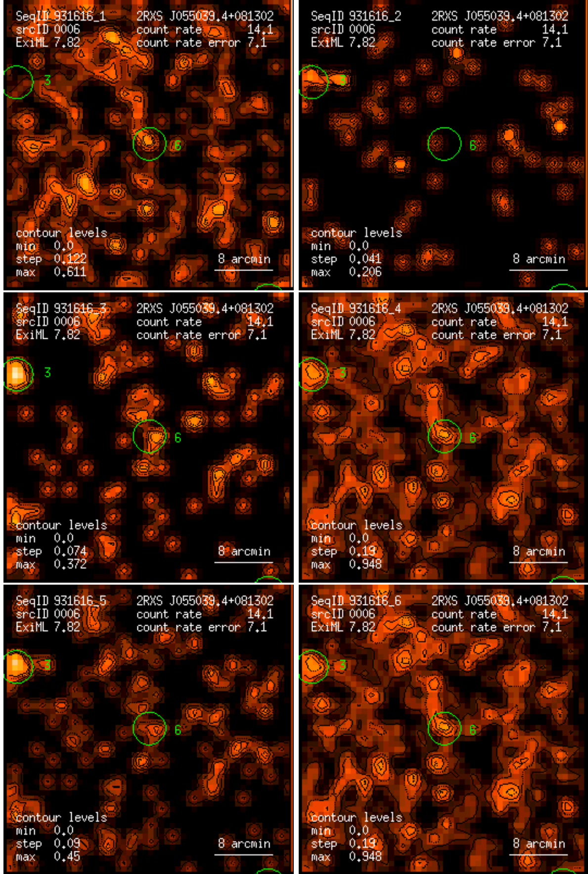
Figure 6: RASS 931616: detection 0006: band rate images, Gaussian filter: (1) PSPC channels 11 – 41, (2) 52 – 90, (3) 91 – 201, (4) 11 – 235, (5) 52 – 201, (6) 11 – 201. Broad band rates in counts/ks. Band rate contour levels in counts/ks/arcmin 2 .
