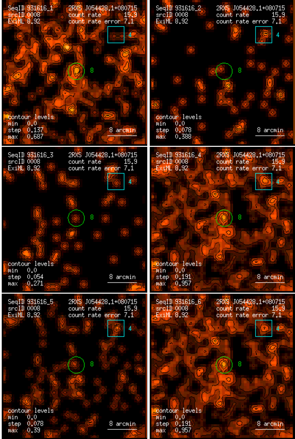
Figure 8: RASS 931616: detection 0008: band rate images, Gaussian filter: (1) PSPC channels 11 – 41, (2) 52 – 90, (3) 91 – 201, (4) 11 – 235, (5) 52 – 201, (6) 11 – 201. Broad band rates in counts/ks. Band rate contour levels in counts/ks/arcmin 2 .
