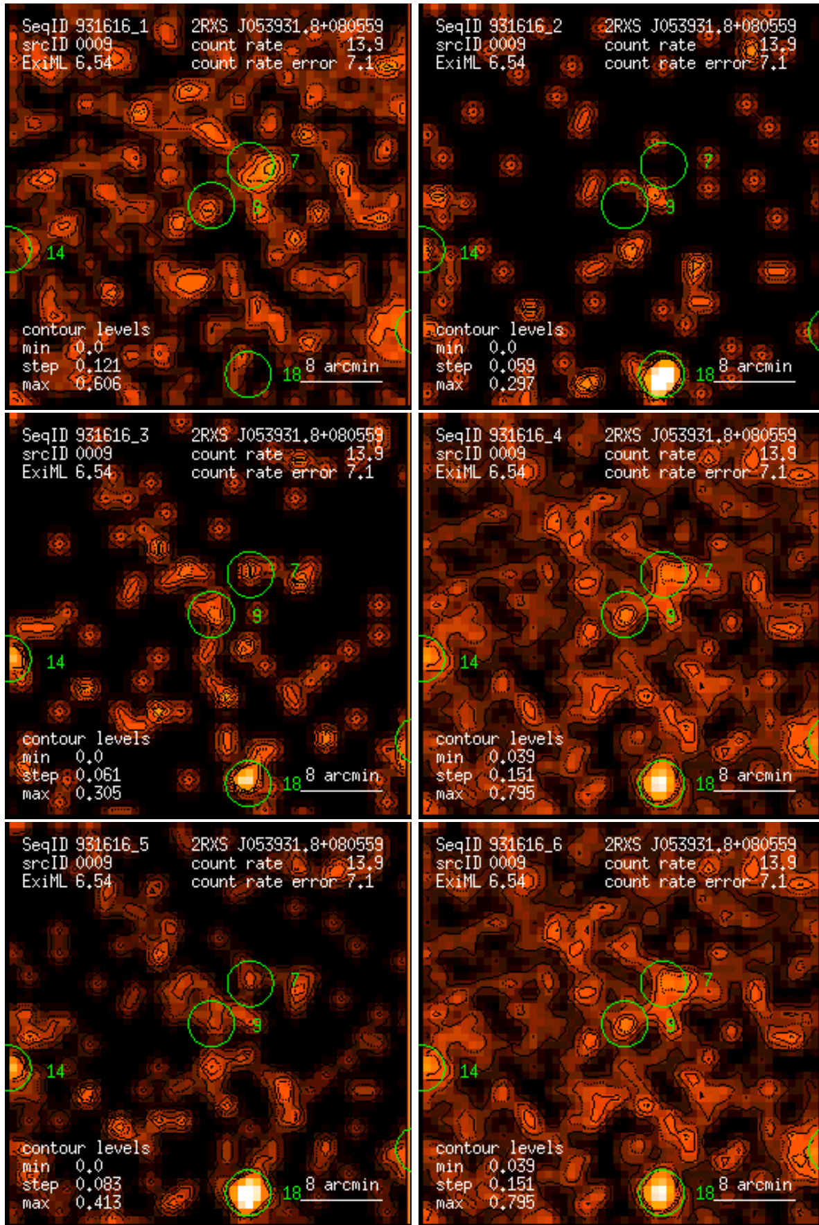
Figure 9: RASS 931616: detection 0009: band rate images, Gaussian filter: (1) PSPC channels 11 – 41, (2) 52 – 90, (3) 91 – 201, (4) 11 – 235, (5) 52 – 201, (6) 11 – 201. Broad band rates in counts/ks. Band rate contour levels in counts/ks/arcmin 2 .
