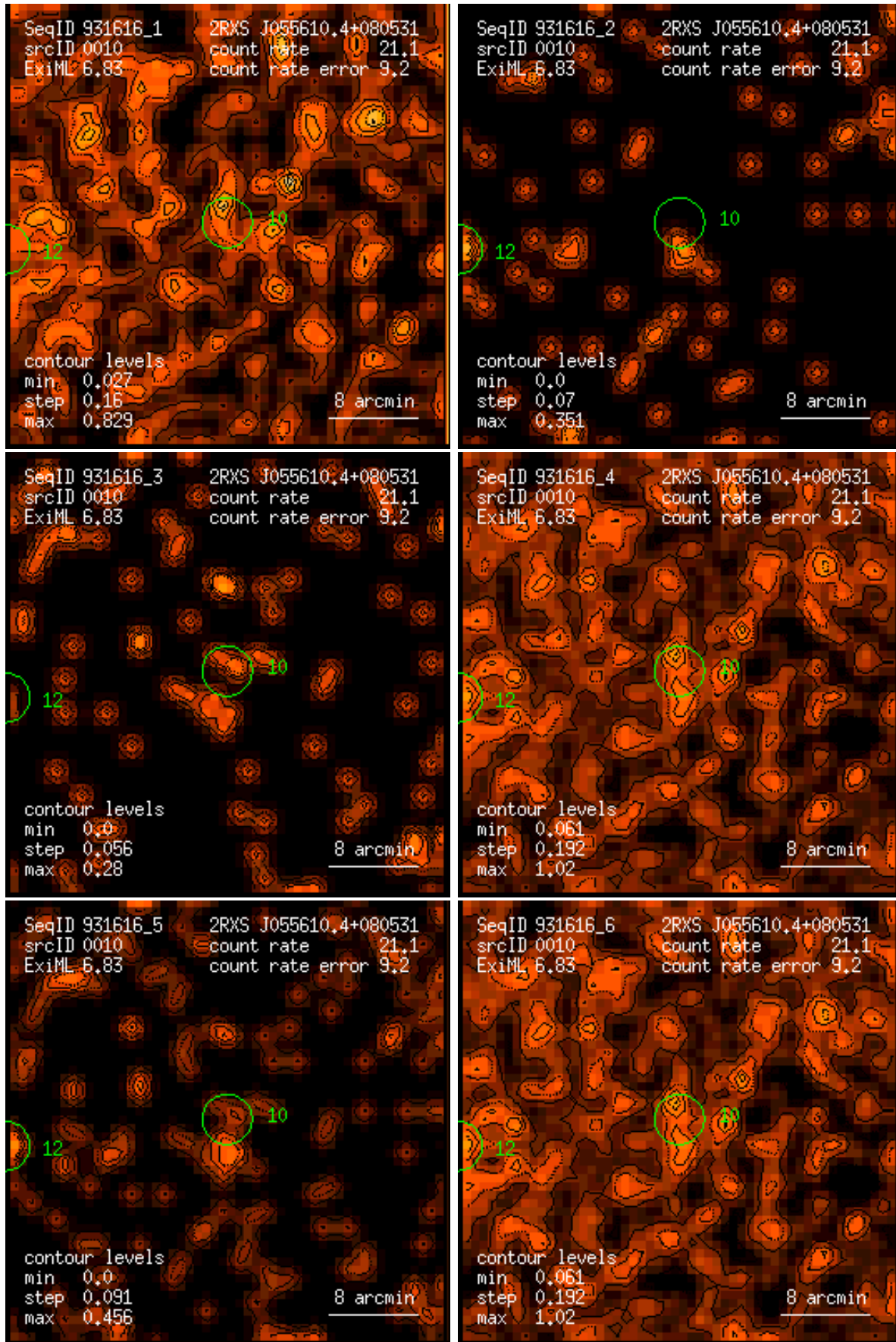
Figure 10: RASS 931616: detection 0010: band rate images, Gaussian filter: (1) PSPC channels 11 – 41, (2) 52 – 90, (3) 91 – 201, (4) 11 – 235, (5) 52 – 201, (6) 11 – 201. Broad band rates in counts/ks. Band rate contour levels in counts/ks/arcmin 2 .
