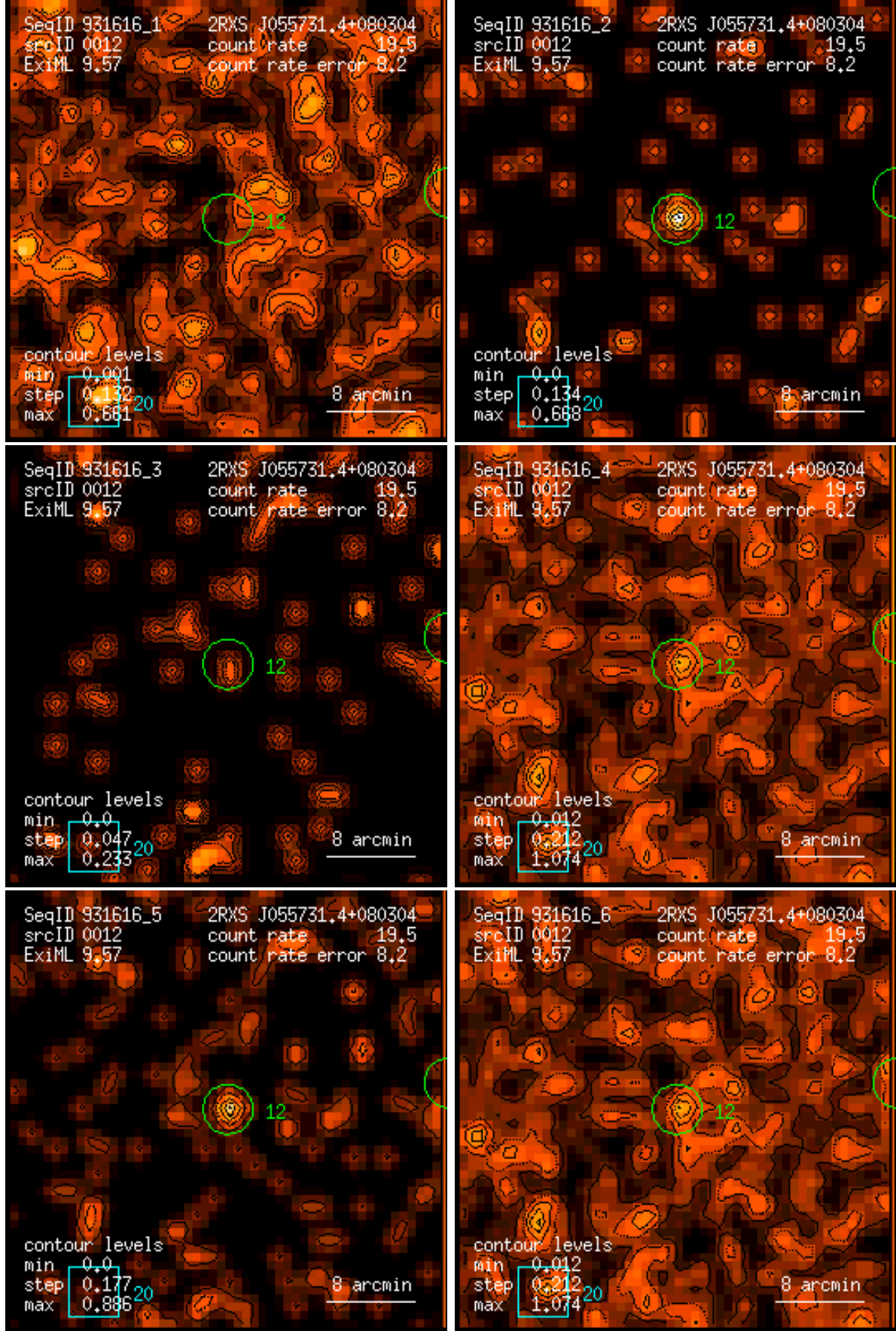
Figure 12: RASS 931616: detection 0012: band rate images, Gaussian filter: (1) PSPC channels 11 – 41, (2) 52 – 90, (3) 91 – 201, (4) 11 – 235, (5) 52 – 201, (6) 11 – 201. Broad band rates in counts/ks. Band rate contour levels in counts/ks/arcmin 2 .
