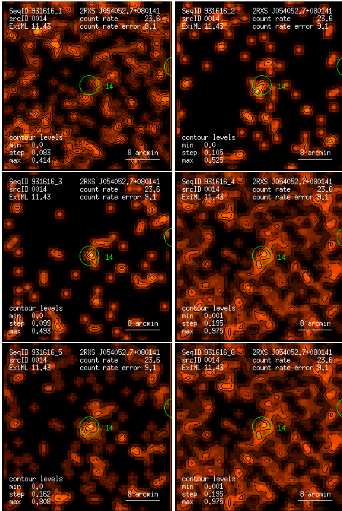
Figure 14: RASS 931616: detection 0014: band rate images, Gaussian filter: (1) PSPC channels 11 – 41, (2) 52 – 90, (3) 91 – 201, (4) 11 – 235, (5) 52 – 201, (6) 11 – 201. Broad band rates in counts/ks. Band rate contour levels in counts/ks/arcmin 2 .
