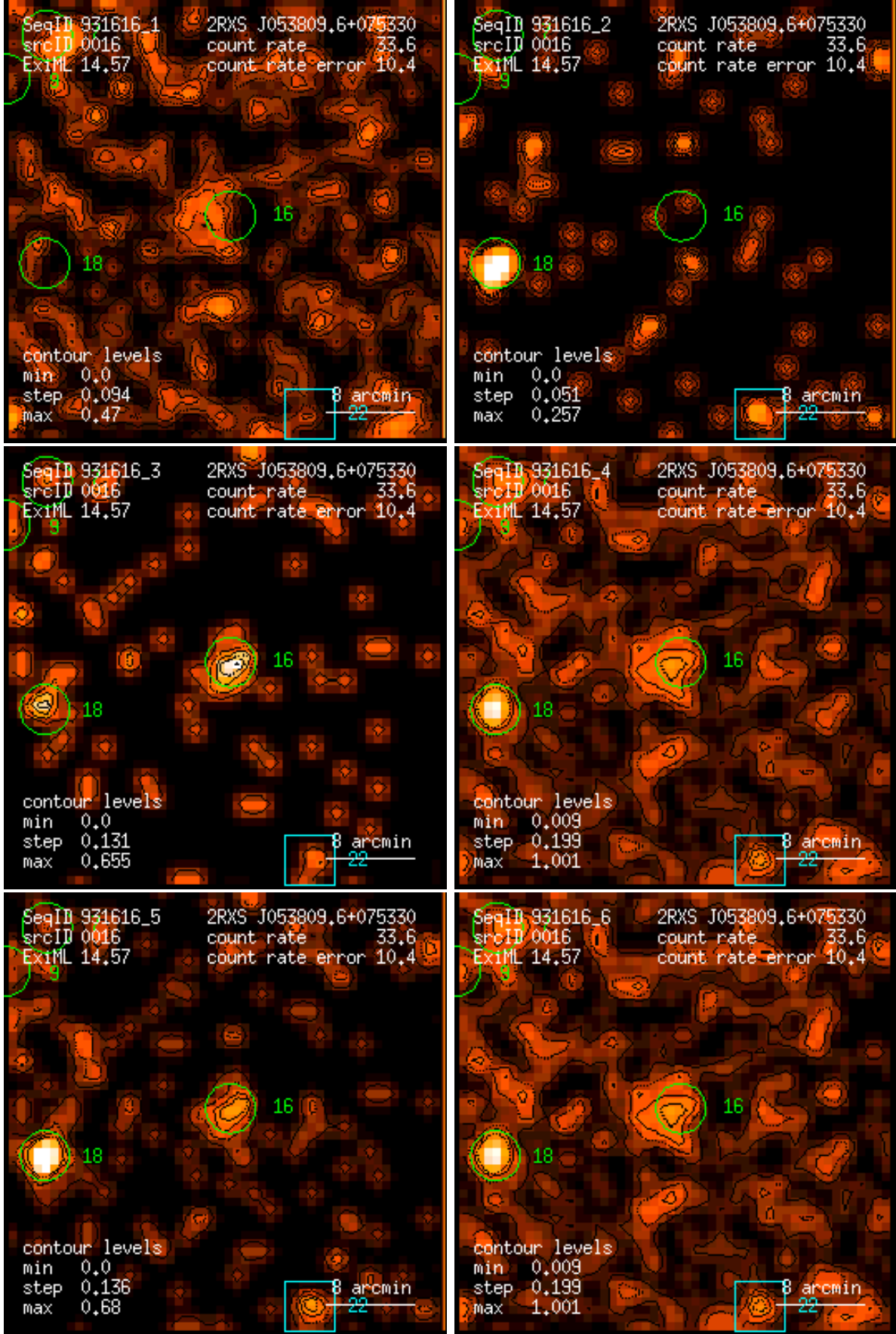
Figure 16: RASS 931616: detection 0016: band rate images, Gaussian filter: (1) PSPC channels 11 – 41, (2) 52 – 90, (3) 91 – 201, (4) 11 – 235, (5) 52 – 201, (6) 11 – 201. Broad band rates in counts/ks. Band rate contour levels in counts/ks/arcmin 2 .
