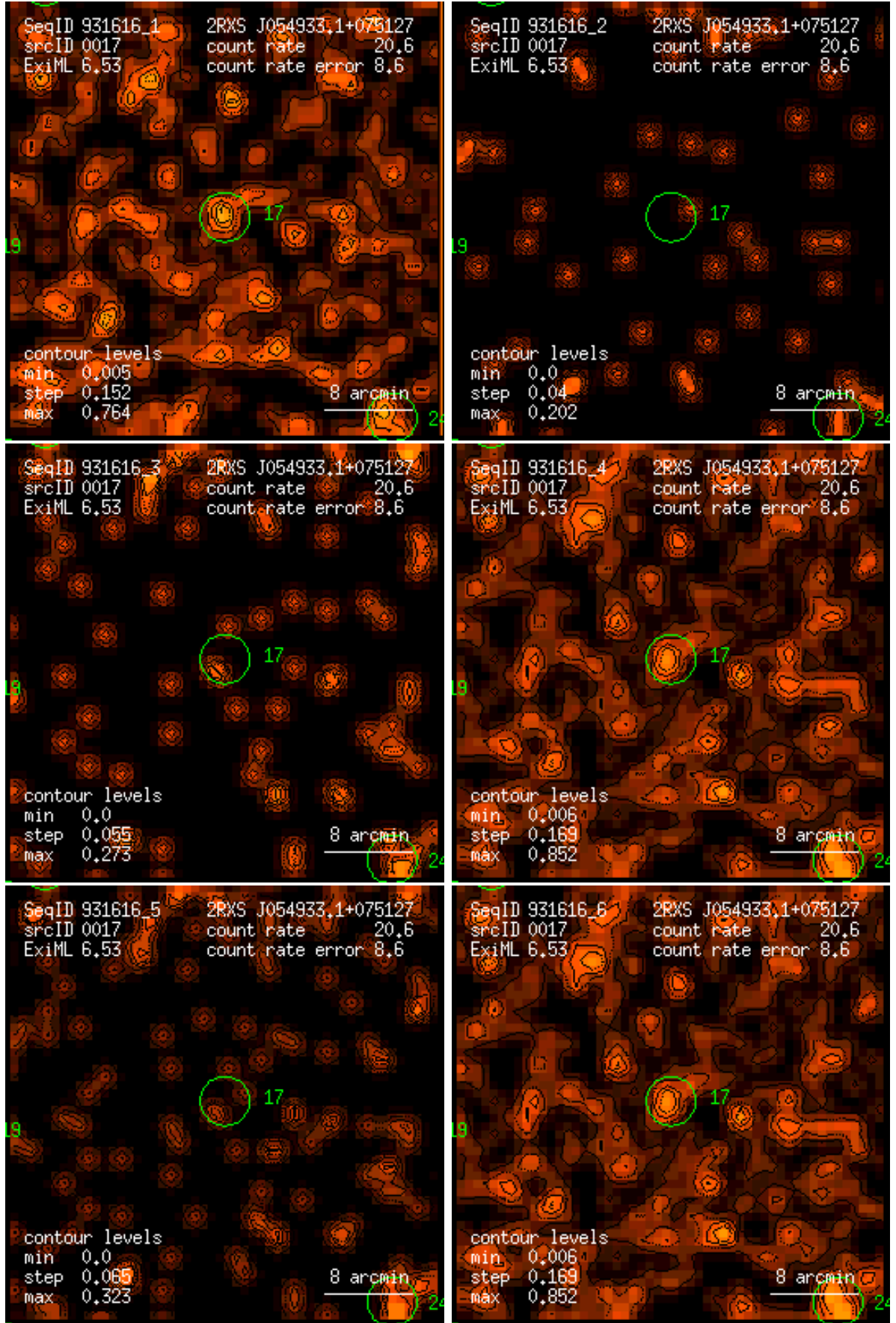
Figure 17: RASS 931616: detection 0017: band rate images, Gaussian filter: (1) PSPC channels 11 – 41, (2) 52 – 90, (3) 91 – 201, (4) 11 – 235, (5) 52 – 201, (6) 11 – 201. Broad band rates in counts/ks. Band rate contour levels in counts/ks/arcmin 2 .
