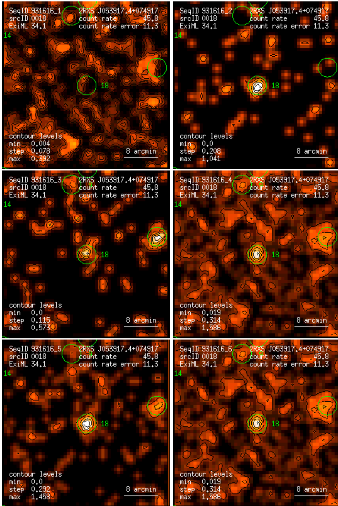
Figure 18: RASS 931616: detection 0018: band rate images, Gaussian filter: (1) PSPC channels 11 – 41, (2) 52 – 90, (3) 91 – 201, (4) 11 – 235, (5) 52 – 201, (6) 11 – 201. Broad band rates in counts/ks. Band rate contour levels in counts/ks/arcmin 2 .
