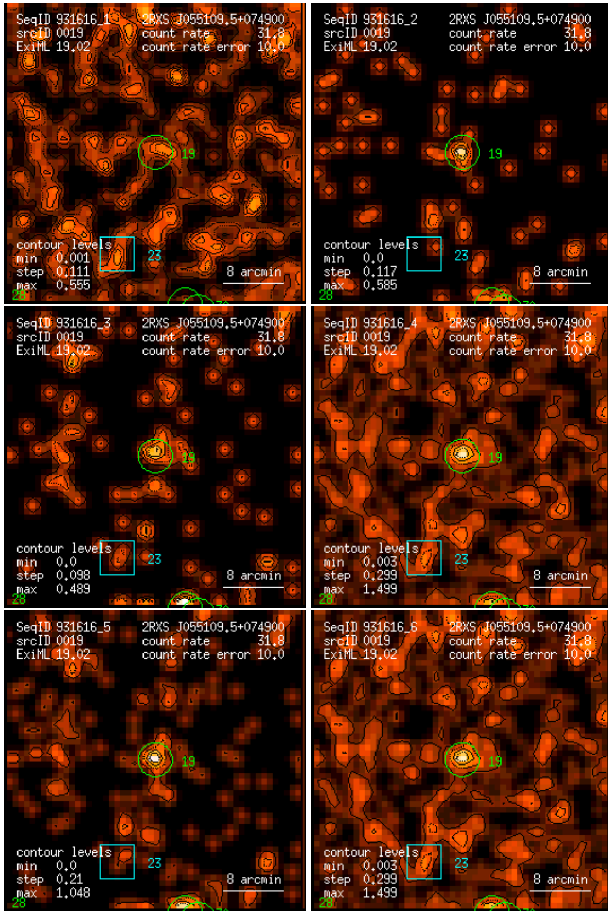
Figure 19: RASS 931616: detection 0019: band rate images, Gaussian filter: (1) PSPC channels 11 – 41, (2) 52 – 90, (3) 91 – 201, (4) 11 – 235, (5) 52 – 201, (6) 11 – 201. Broad band rates in counts/ks. Band rate contour levels in counts/ks/arcmin 2 .
