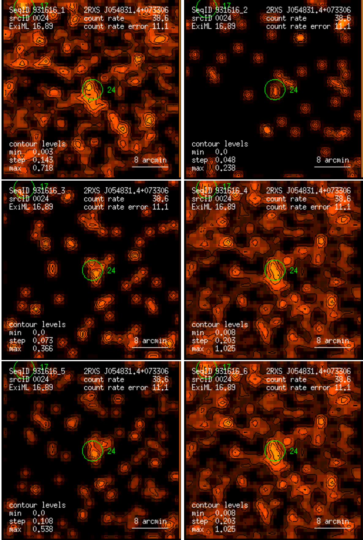
Figure 24: RASS 931616: detection 0024: band rate images, Gaussian filter: (1) PSPC channels 11 – 41, (2) 52 – 90, (3) 91 – 201, (4) 11 – 235, (5) 52 – 201, (6) 11 – 201. Broad band rates in counts/ks. Band rate contour levels in counts/ks/arcmin 2 .
