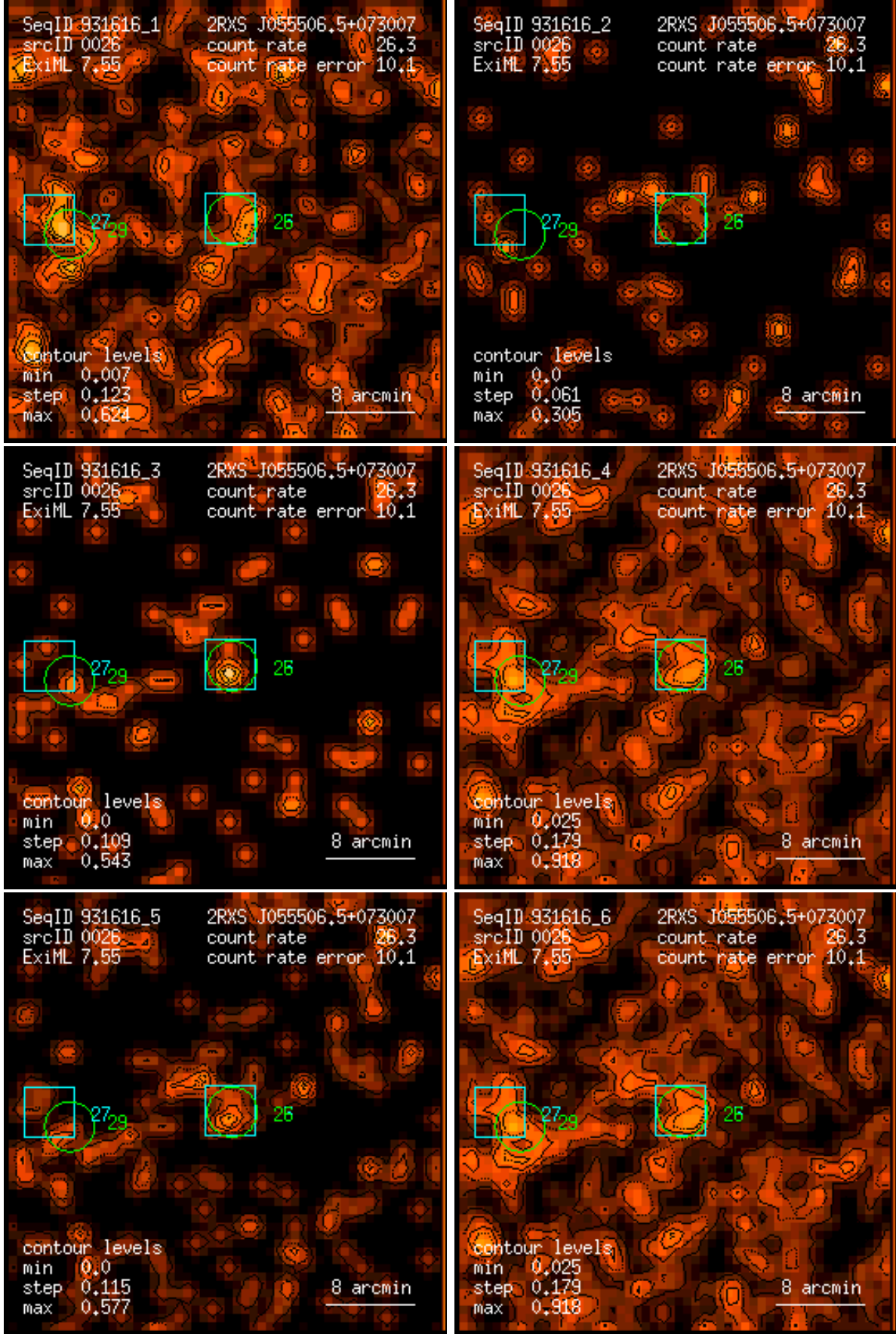
Figure 26: RASS 931616: detection 0026: band rate images, Gaussian filter: (1) PSPC channels 11 – 41, (2) 52 – 90, (3) 91 – 201, (4) 11 – 235, (5) 52 – 201, (6) 11 – 201. Broad band rates in counts/ks. Band rate contour levels in counts/ks/arcmin 2 .
