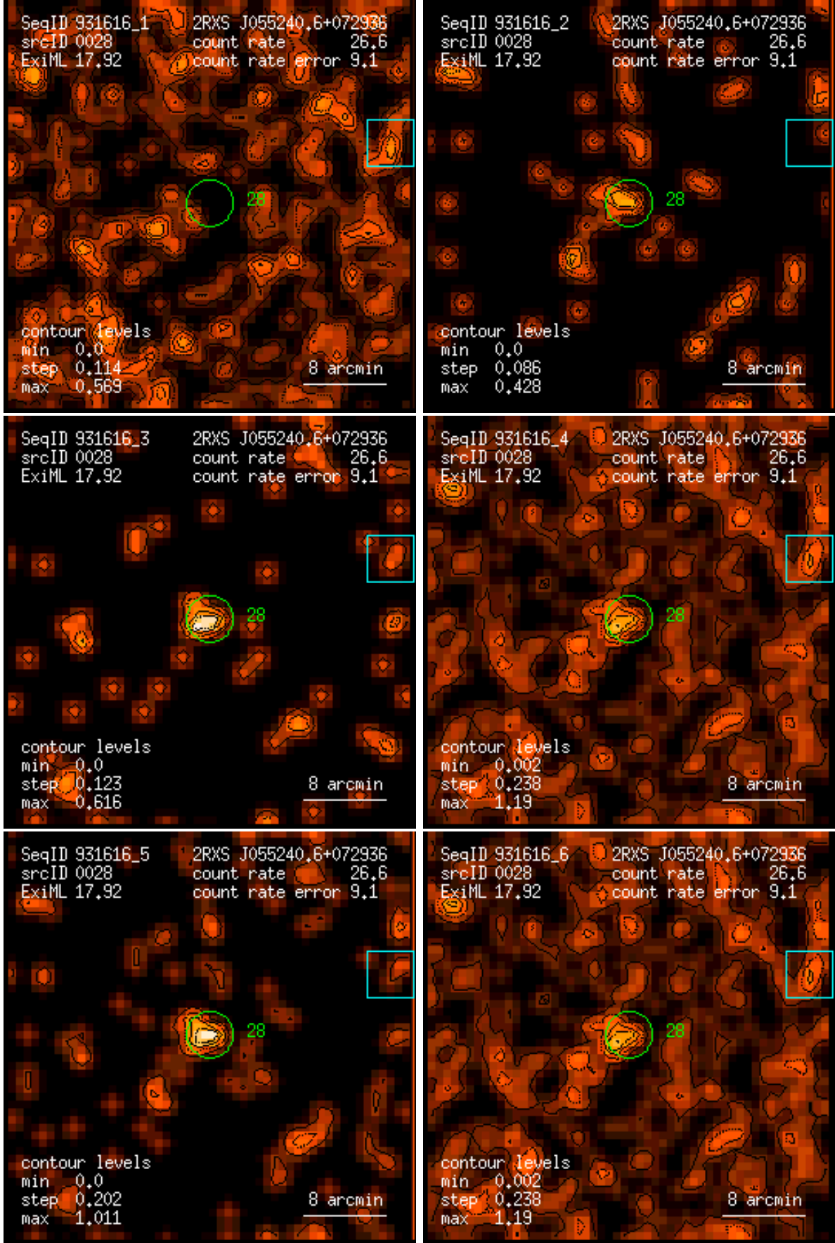
Figure 28: RASS 931616: detection 0028: band rate images, Gaussian filter: (1) PSPC channels 11 – 41, (2) 52 – 90, (3) 91 – 201, (4) 11 – 235, (5) 52 – 201, (6) 11 – 201. Broad band rates in counts/ks. Band rate contour levels in counts/ks/arcmin 2 .
