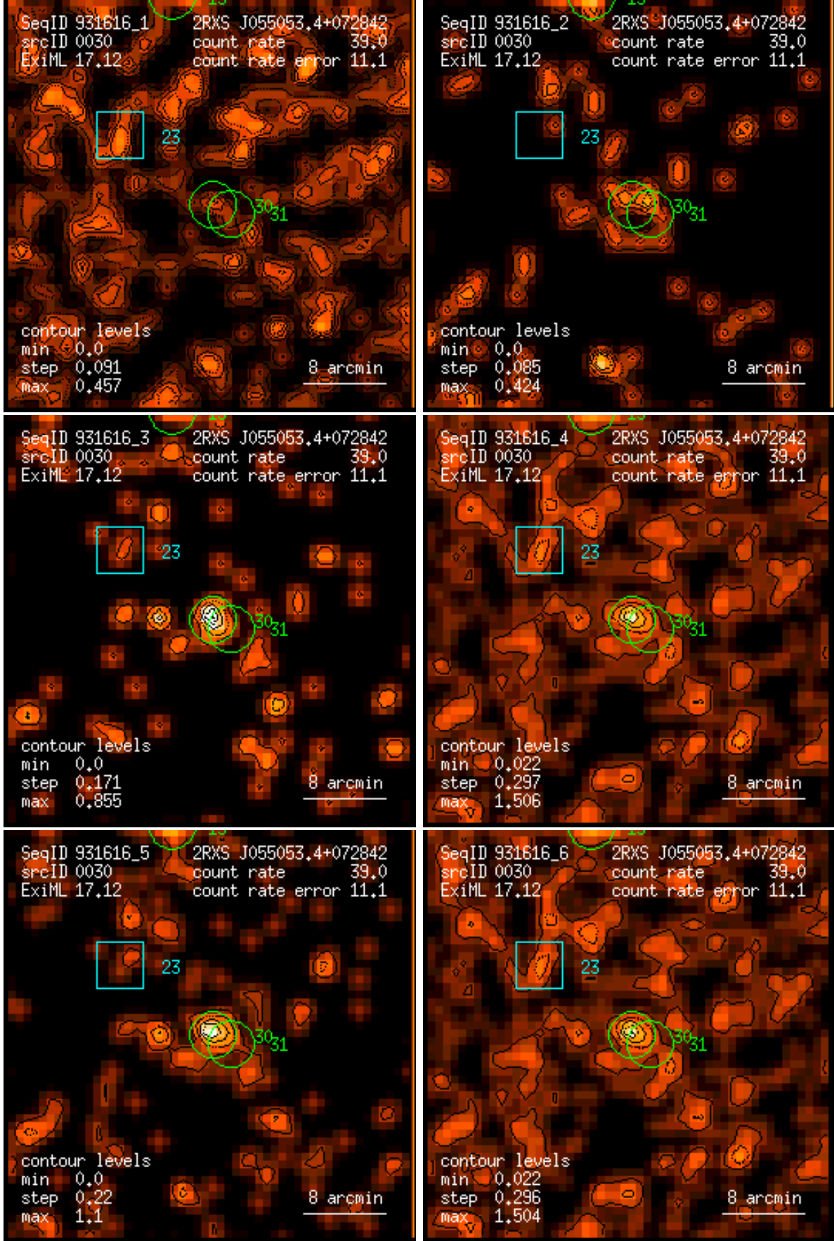
Figure 30: RASS 931616: detection 0030: band rate images, Gaussian filter: (1) PSPC channels 11 – 41, (2) 52 – 90, (3) 91 – 201, (4) 11 – 235, (5) 52 – 201, (6) 11 – 201. Broad band rates in counts/ks. Band rate contour levels in counts/ks/arcmin 2 .
