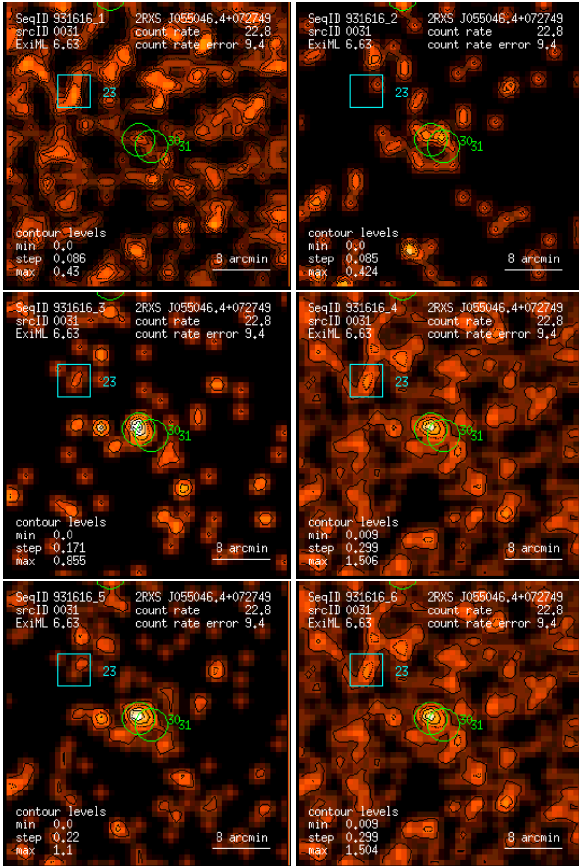
Figure 31: RASS 931616: detection 0031: band rate images, Gaussian filter: (1) PSPC channels 11 – 41, (2) 52 – 90, (3) 91 – 201, (4) 11 – 235, (5) 52 – 201, (6) 11 – 201. Broad band rates in counts/ks. Band rate contour levels in counts/ks/arcmin 2 .
