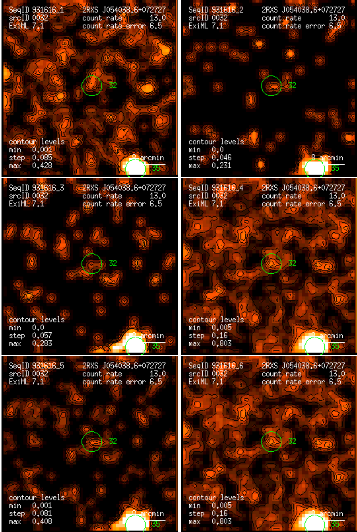
Figure 32: RASS 931616: detection 0032: band rate images, Gaussian filter: (1) PSPC channels 11 – 41, (2) 52 – 90, (3) 91 – 201, (4) 11 – 235, (5) 52 – 201, (6) 11 – 201. Broad band rates in counts/ks. Band rate contour levels in counts/ks/arcmin 2 .
