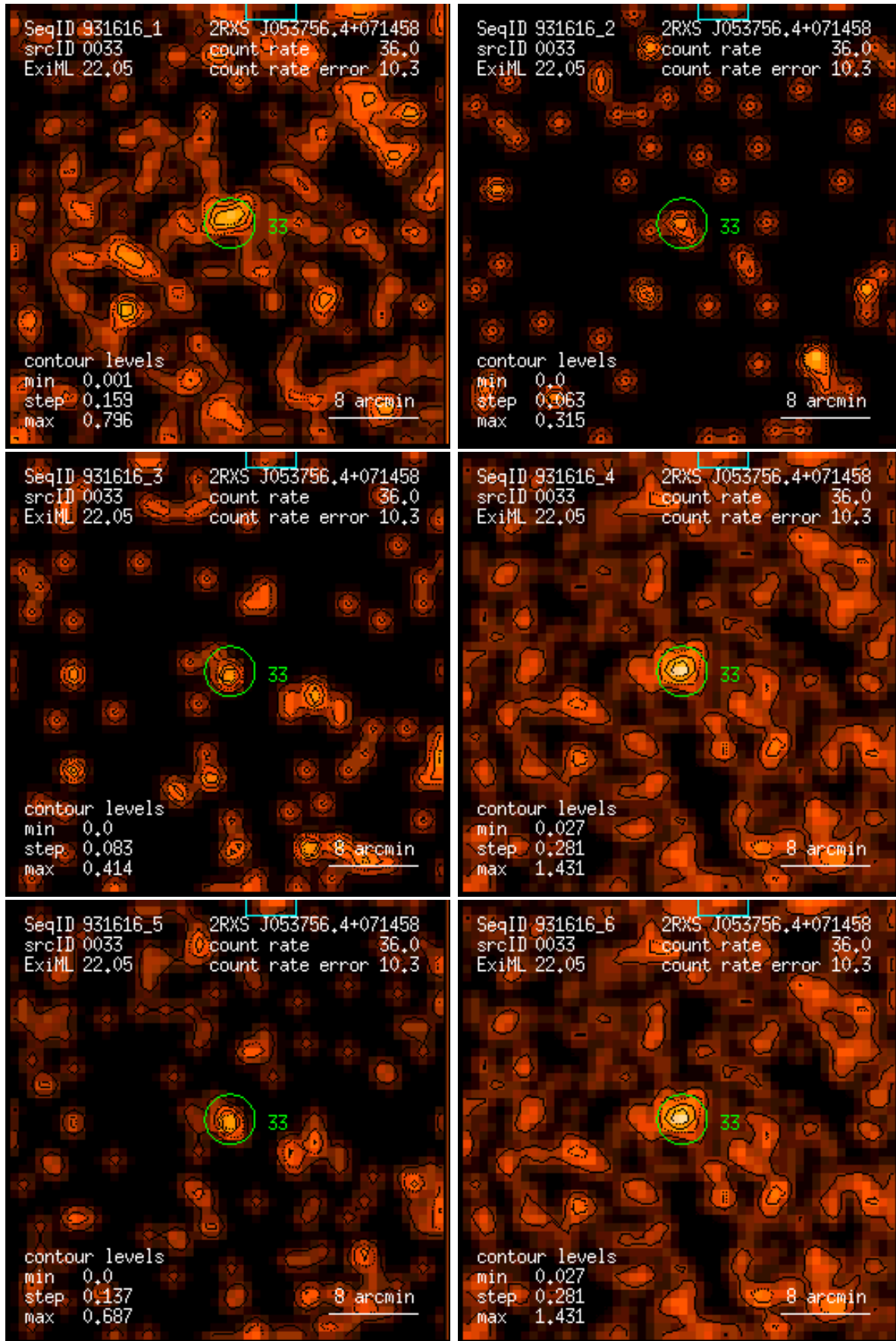
Figure 33: RASS 931616: detection 0033: band rate images, Gaussian filter: (1) PSPC channels 11 – 41, (2) 52 – 90, (3) 91 – 201, (4) 11 – 235, (5) 52 – 201, (6) 11 – 201. Broad band rates in counts/ks. Band rate contour levels in counts/ks/arcmin 2 .
