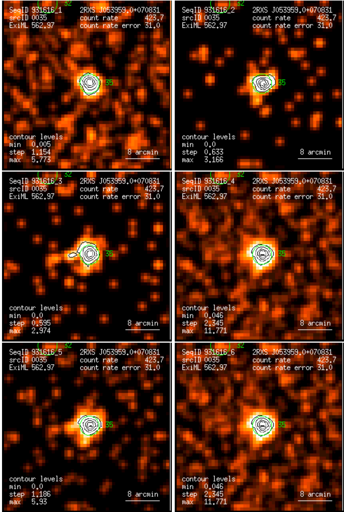
Figure 35: RASS 931616: detection 0035: band rate images, Gaussian filter: (1) PSPC channels 11 – 41, (2) 52 – 90, (3) 91 – 201, (4) 11 – 235, (5) 52 – 201, (6) 11 – 201. Broad band rates in counts/ks. Band rate contour levels in counts/ks/arcmin 2 .
