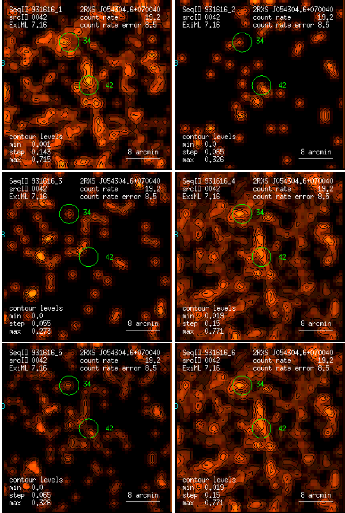
Figure 42: RASS 931616: detection 0042: band rate images, Gaussian filter: (1) PSPC channels 11 – 41, (2) 52 – 90, (3) 91 – 201, (4) 11 – 235, (5) 52 – 201, (6) 11 – 201. Broad band rates in counts/ks. Band rate contour levels in counts/ks/arcmin 2 .
