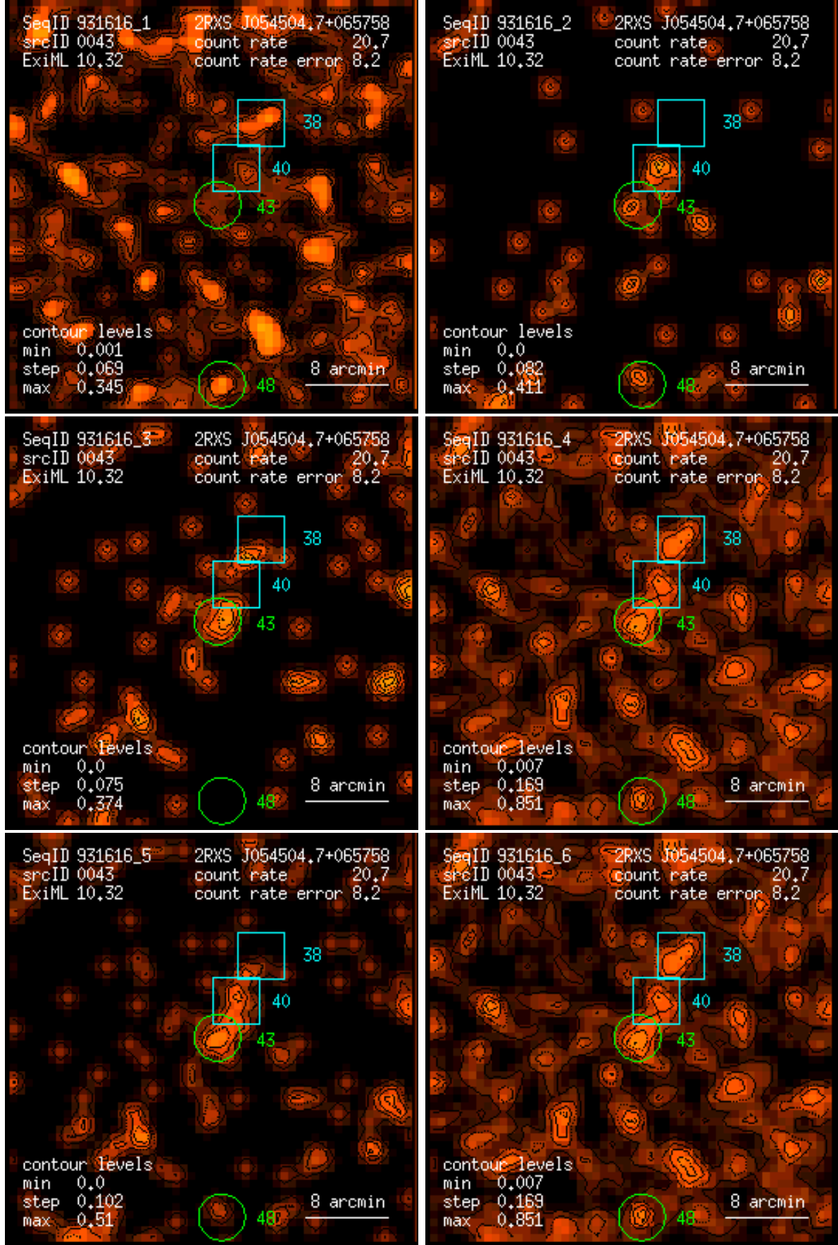
Figure 43: RASS 931616: detection 0043: band rate images, Gaussian filter: (1) PSPC channels 11 – 41, (2) 52 – 90, (3) 91 – 201, (4) 11 – 235, (5) 52 – 201, (6) 11 – 201. Broad band rates in counts/ks. Band rate contour levels in counts/ks/arcmin 2 .
