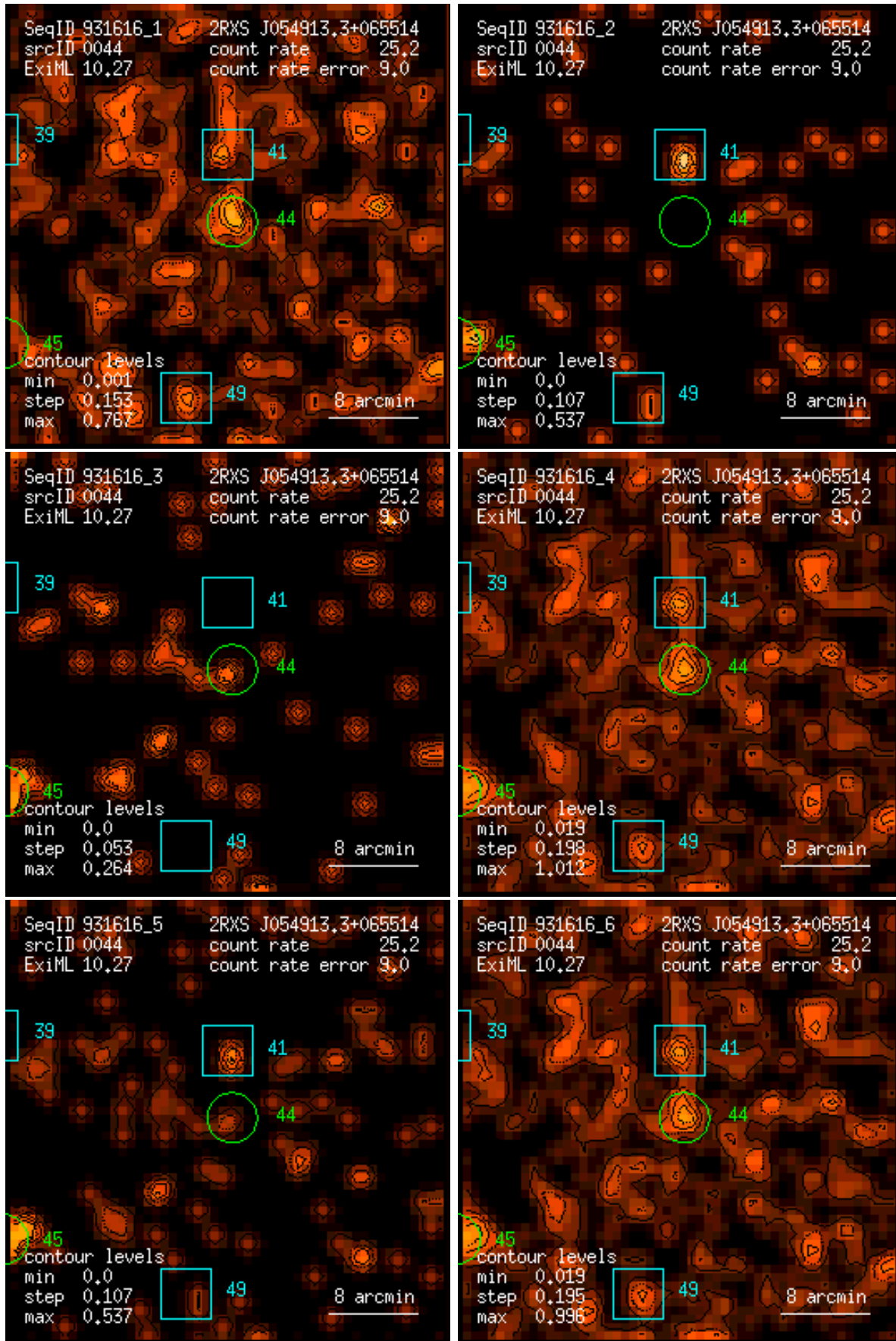
Figure 44: RASS 931616: detection 0044: band rate images, Gaussian filter: (1) PSPC channels 11 – 41, (2) 52 – 90, (3) 91 – 201, (4) 11 – 235, (5) 52 – 201, (6) 11 – 201. Broad band rates in counts/ks. Band rate contour levels in counts/ks/arcmin 2 .
