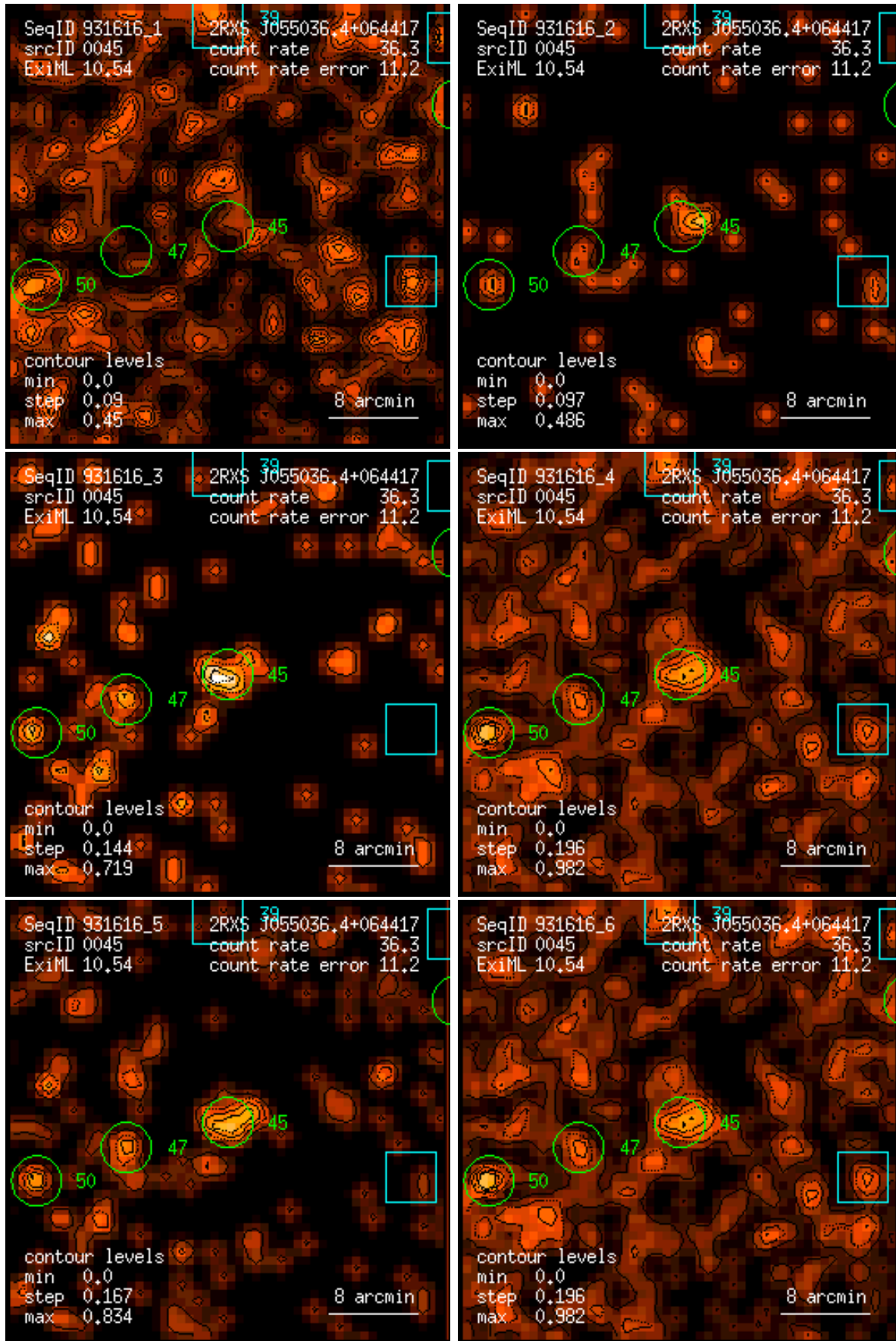
Figure 45: RASS 931616: detection 0045: band rate images, Gaussian filter: (1) PSPC channels 11 – 41, (2) 52 – 90, (3) 91 – 201, (4) 11 – 235, (5) 52 – 201, (6) 11 – 201. Broad band rates in counts/ks. Band rate contour levels in counts/ks/arcmin 2 .
