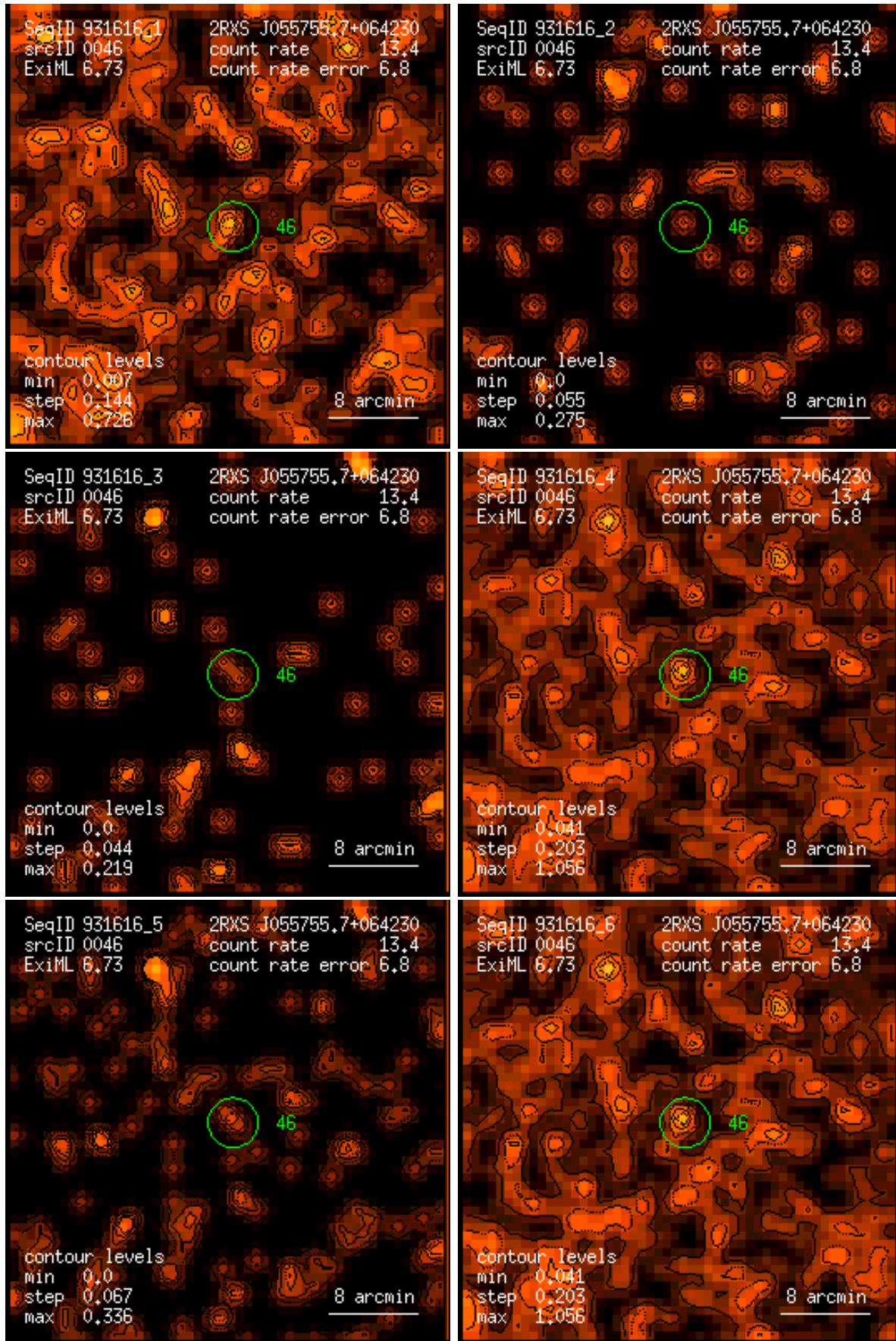
Figure 46: RASS 931616: detection 0046: band rate images, Gaussian filter: (1) PSPC channels 11 – 41, (2) 52 – 90, (3) 91 – 201, (4) 11 – 235, (5) 52 – 201, (6) 11 – 201. Broad band rates in counts/ks. Band rate contour levels in counts/ks/arcmin 2 .
