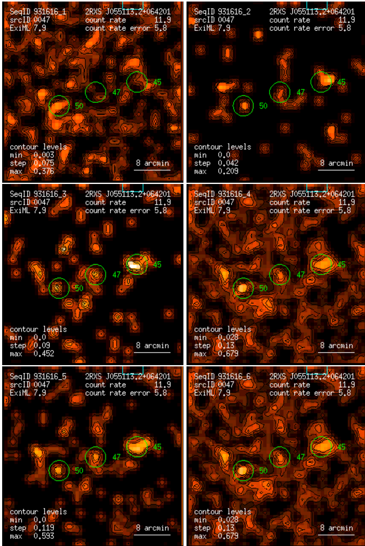
Figure 47: RASS 931616: detection 0047: band rate images, Gaussian filter: (1) PSPC channels 11 – 41, (2) 52 – 90, (3) 91 – 201, (4) 11 – 235, (5) 52 – 201, (6) 11 – 201. Broad band rates in counts/ks. Band rate contour levels in counts/ks/arcmin 2 .
