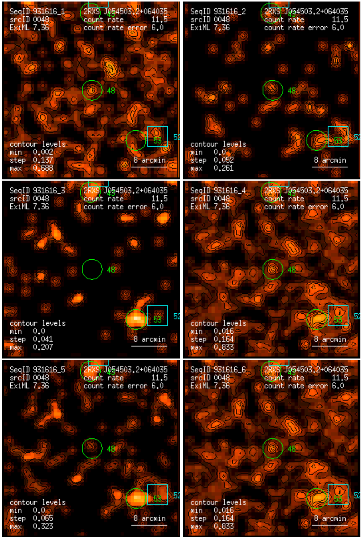
Figure 48: RASS 931616: detection 0048: band rate images, Gaussian filter: (1) PSPC channels 11 – 41, (2) 52 – 90, (3) 91 – 201, (4) 11 – 235, (5) 52 – 201, (6) 11 – 201. Broad band rates in counts/ks. Band rate contour levels in counts/ks/arcmin 2 .
