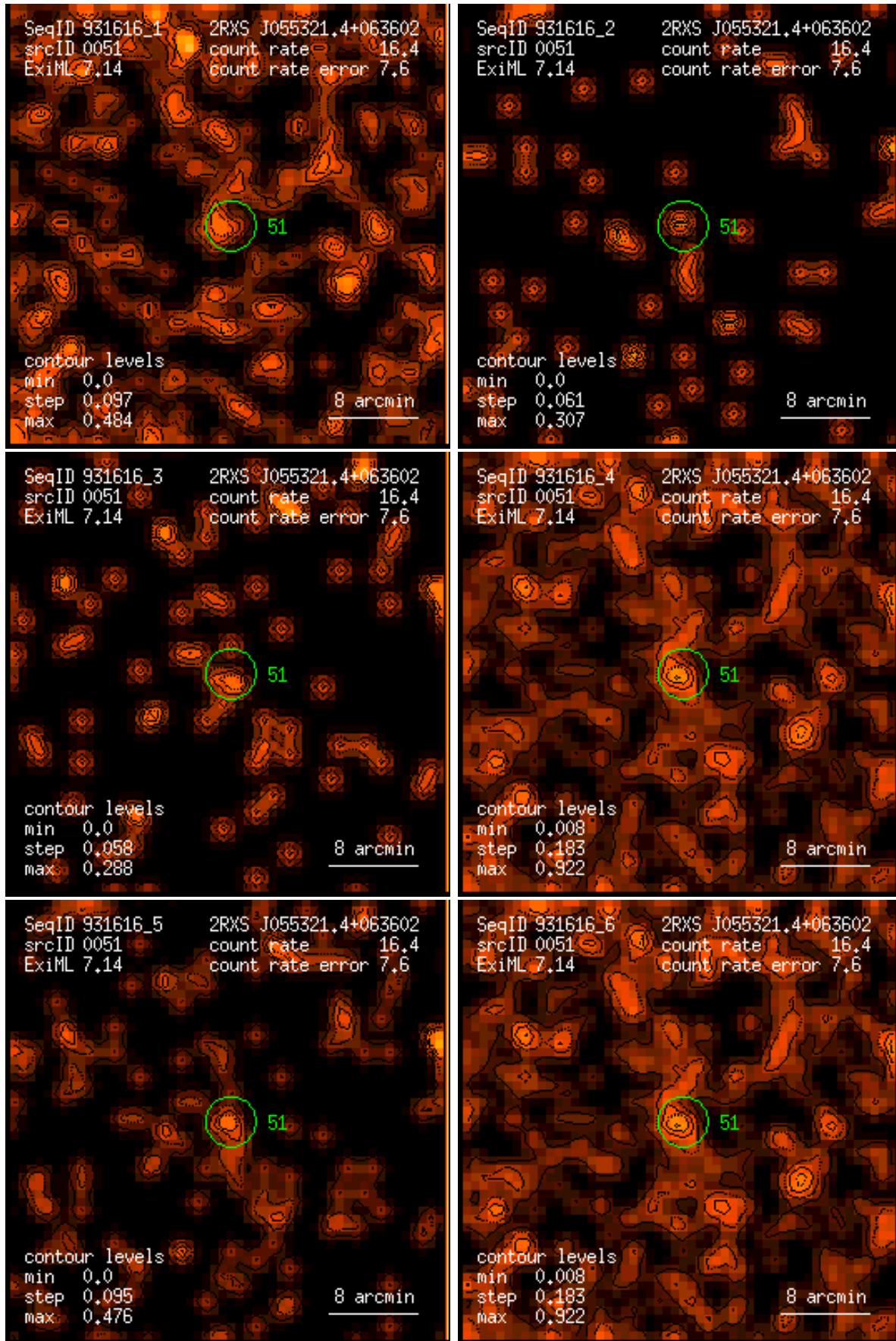
Figure 51: RASS 931616: detection 0051: band rate images, Gaussian filter: (1) PSPC channels 11 – 41, (2) 52 – 90, (3) 91 – 201, (4) 11 – 235, (5) 52 – 201, (6) 11 – 201. Broad band rates in counts/ks. Band rate contour levels in counts/ks/arcmin 2 .
