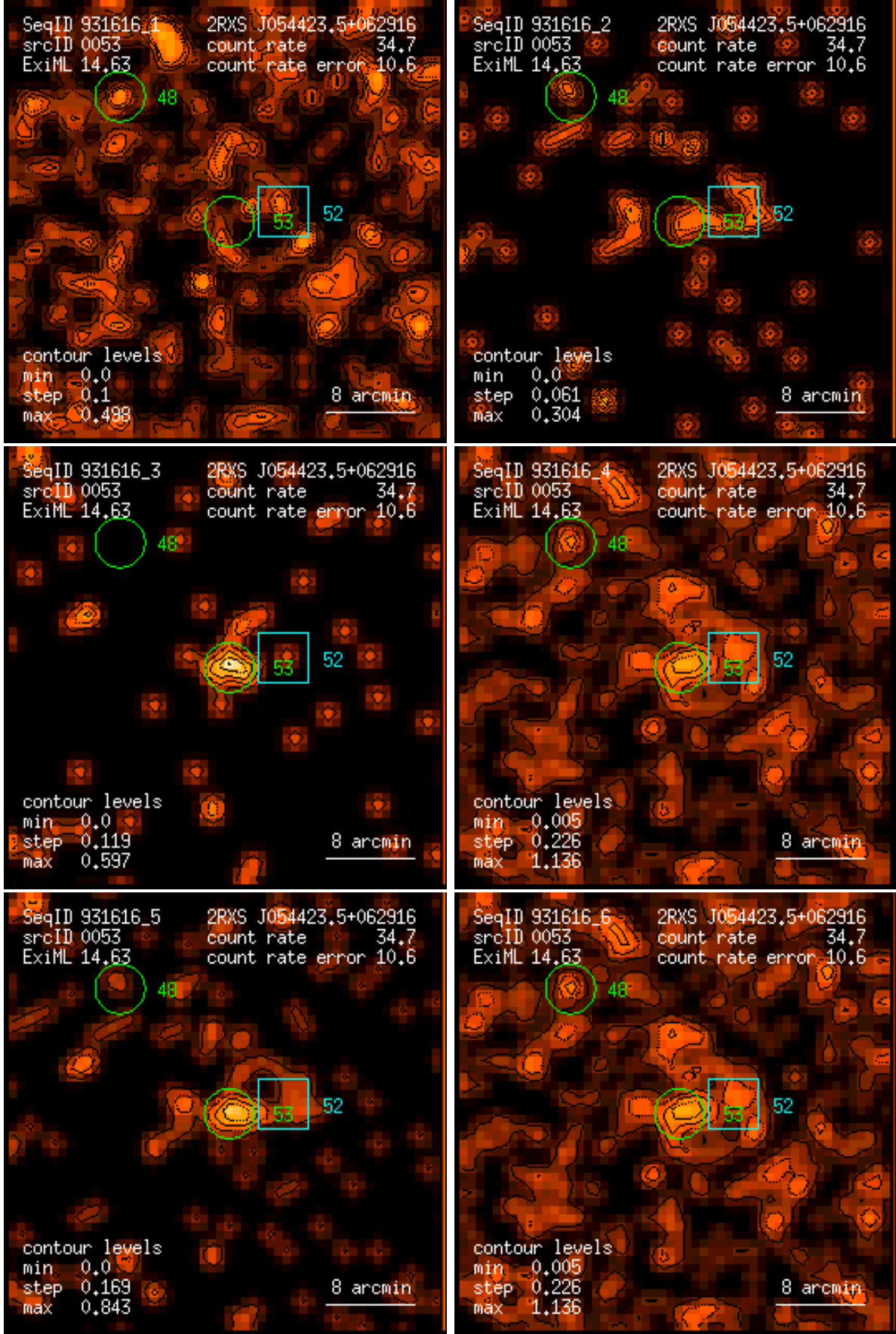
Figure 53: RASS 931616: detection 0053: band rate images, Gaussian filter: (1) PSPC channels 11 – 41, (2) 52 – 90, (3) 91 – 201, (4) 11 – 235, (5) 52 – 201, (6) 11 – 201. Broad band rates in counts/ks. Band rate contour levels in counts/ks/arcmin 2 .
